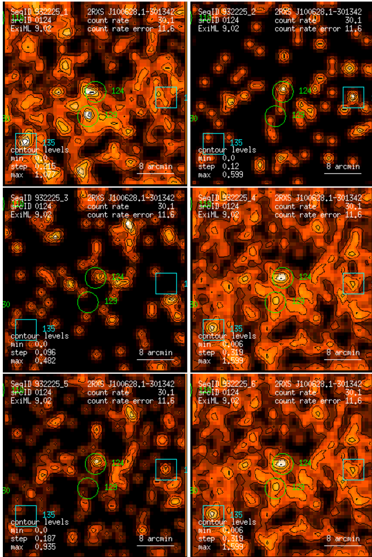
Figure 124: RASS 932225: detection 0124: band rate images, Gaussian filter: (1) PSPC channels 11 – 41, (2) 52 – 90, (3) 91 – 201, (4) 11 – 235, (5) 52 – 201, (6) 11 – 201. Broad band rates in counts/ks. Band rate contour levels in counts/ks/arcmin 2 .
