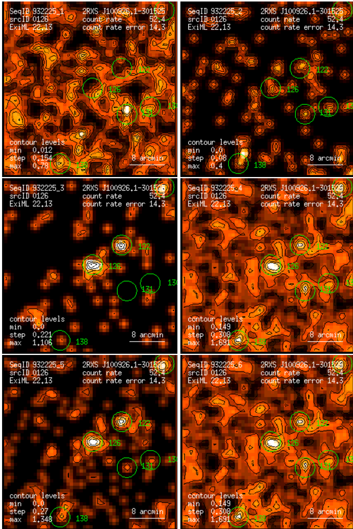
Figure 126: RASS 932225: detection 0126: band rate images, Gaussian filter: (1) PSPC channels 11 – 41, (2) 52 – 90, (3) 91 – 201, (4) 11 – 235, (5) 52 – 201, (6) 11 – 201. Broad band rates in counts/ks. Band rate contour levels in counts/ks/arcmin 2 .
