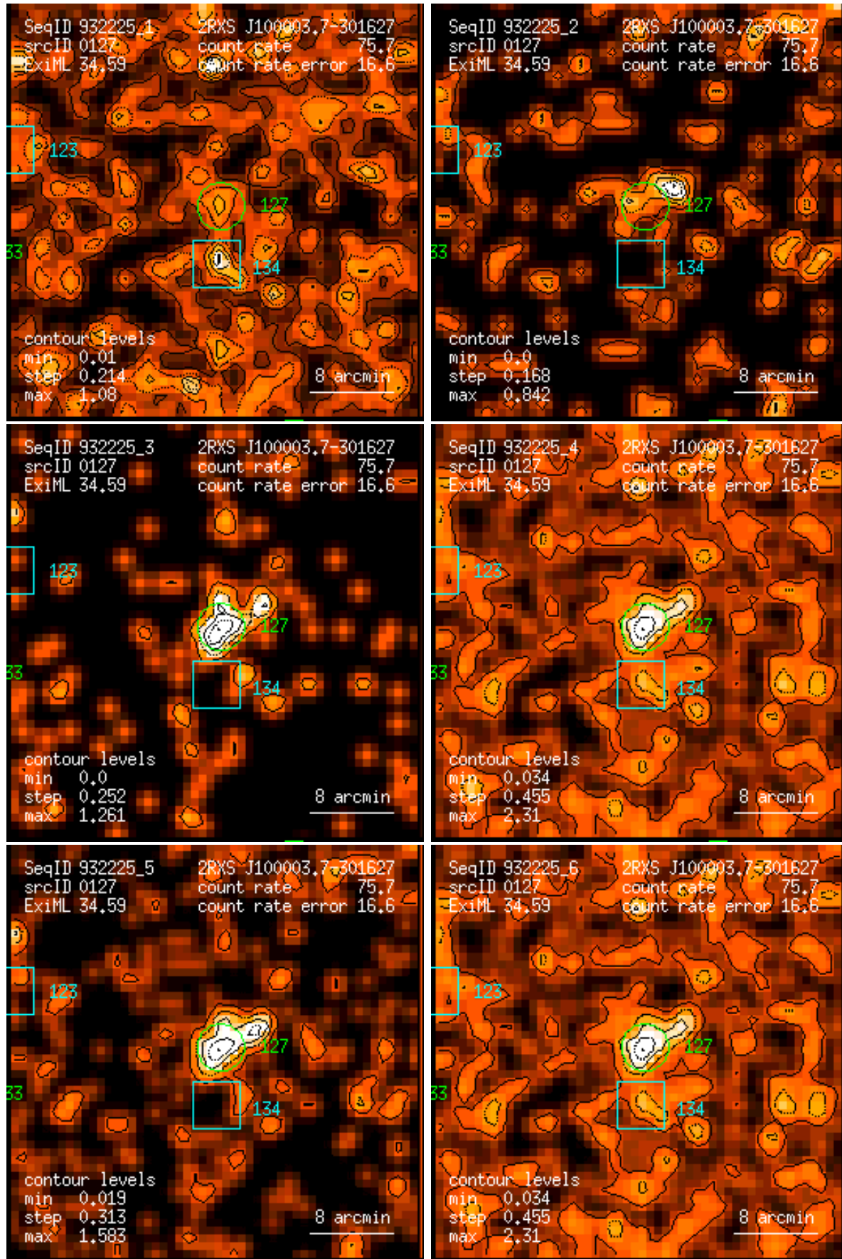
Figure 127: RASS 932225: detection 0127: band rate images, Gaussian filter: (1) PSPPC channels 11 – 41, (2) 52 – 90, (3) 91 – 201, (4) 11 – 235, (5) 52 – 201, (6) 11 – 201. Broad band rates in counts/ks. Band rate contour levels in counts/ks/arcmin 2 .
