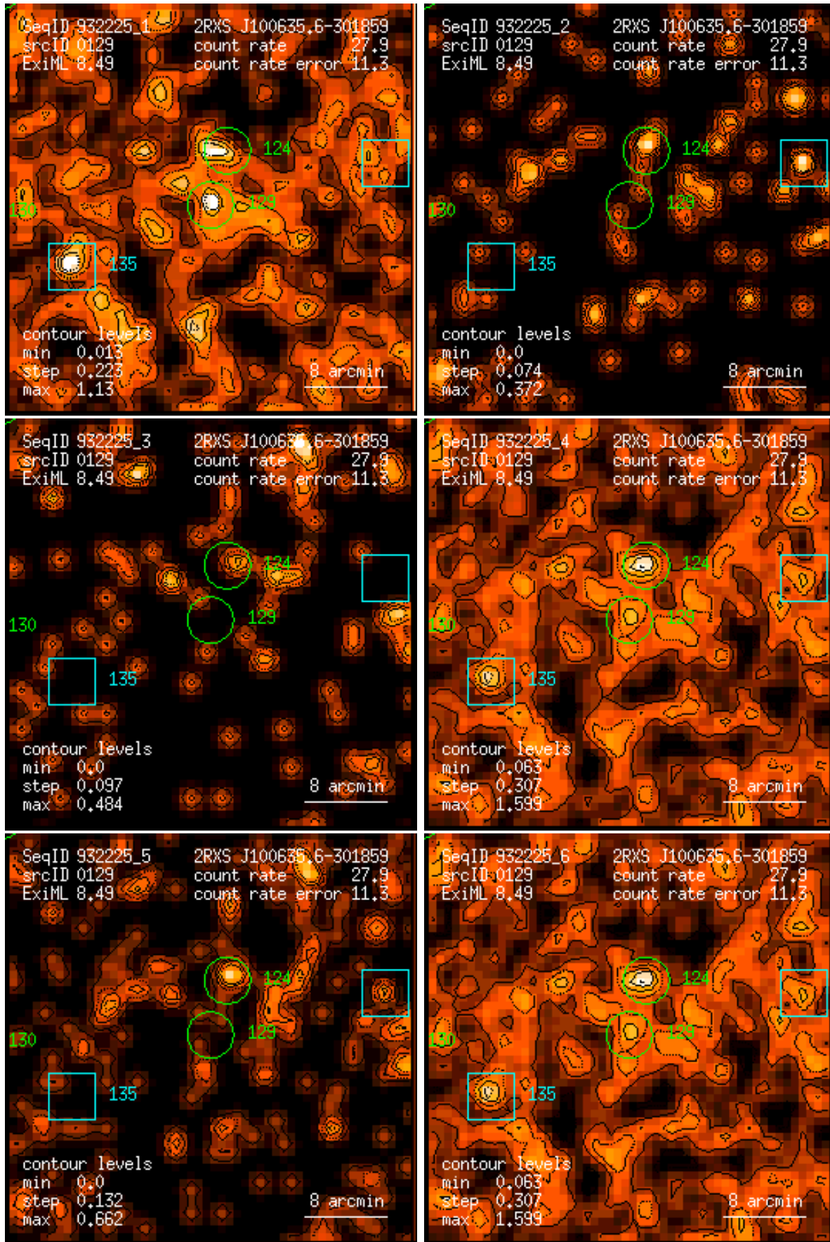
Figure 129: RASS 932225: detection 0129: band rate images, Gaussian filter: (1) PSPC channels 11 – 41, (2) 52 – 90, (3) 91 – 201, (4) 11 – 235, (5) 52 – 201, (6) 11 – 201. Broad band rates in counts/ks. Band rate contour levels in counts/ks/arcmin 2 .
