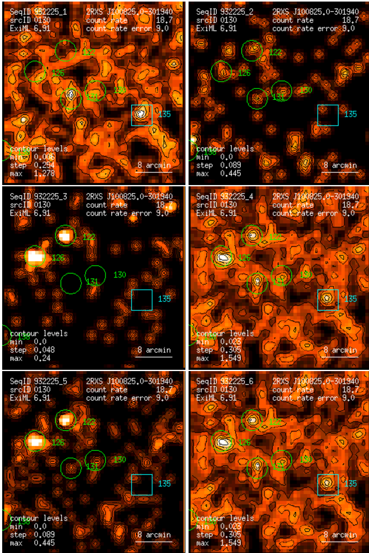
Figure 130: RASS 932225: detection 0130: band rate images, Gaussian filter: (1) PSPC channels 11 – 41, (2) 52 – 90, (3) 91 – 201, (4) 11 – 235, (5) 52 – 201, (6) 11 – 201. Broad band rates in counts/ks. Band rate contour levels in counts/ks/arcmin 2 .
