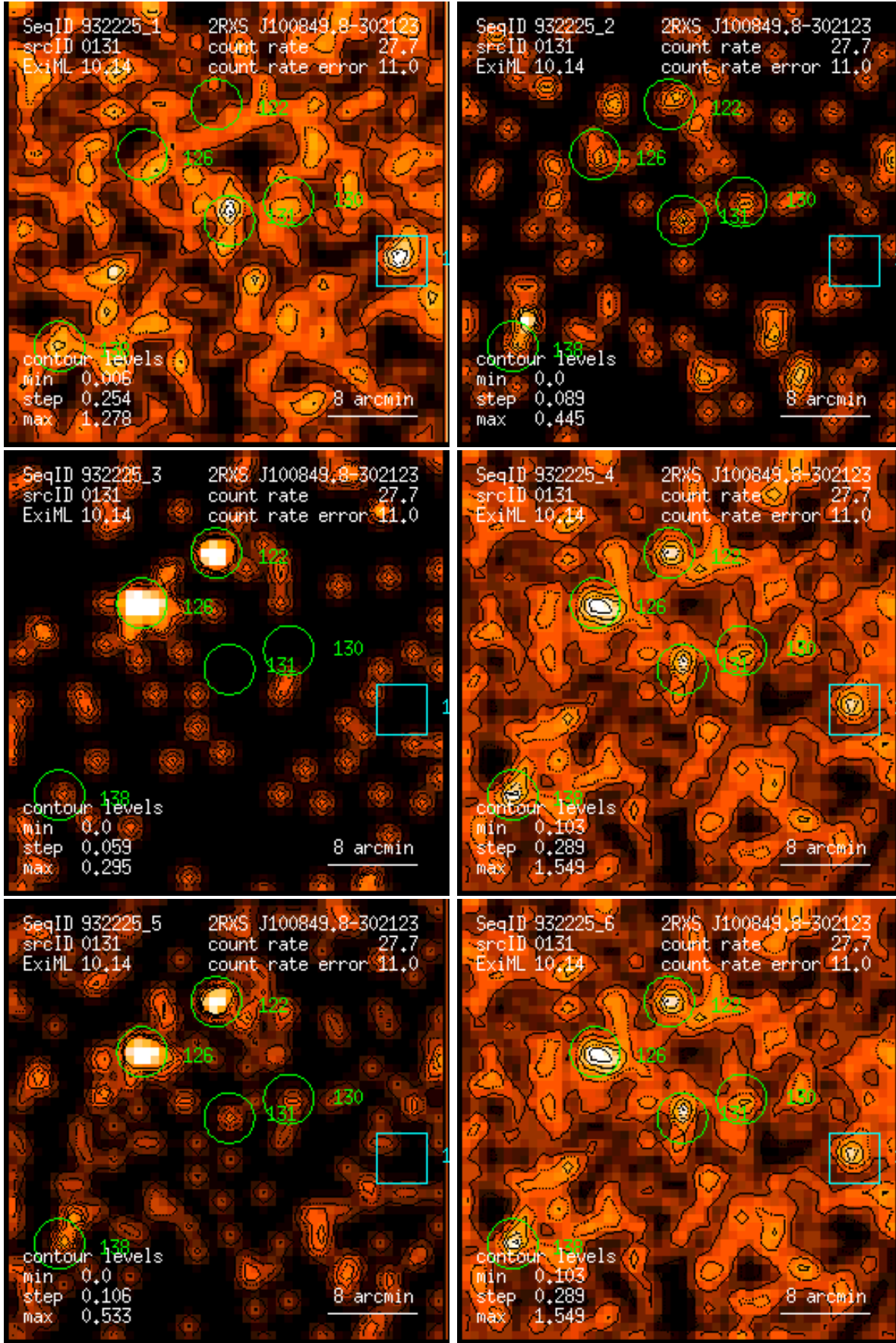
Figure 131: RASS 932225: detection 0131: band rate images, Gaussian filter: (1) PSPC channels 11 – 41, (2) 52 – 90, (3) 91 – 201, (4) 11 – 235, (5) 52 – 201, (6) 11 – 201. Broad band rates in counts/ks. Band rate contour levels in counts/ks/arcmin 2 .
