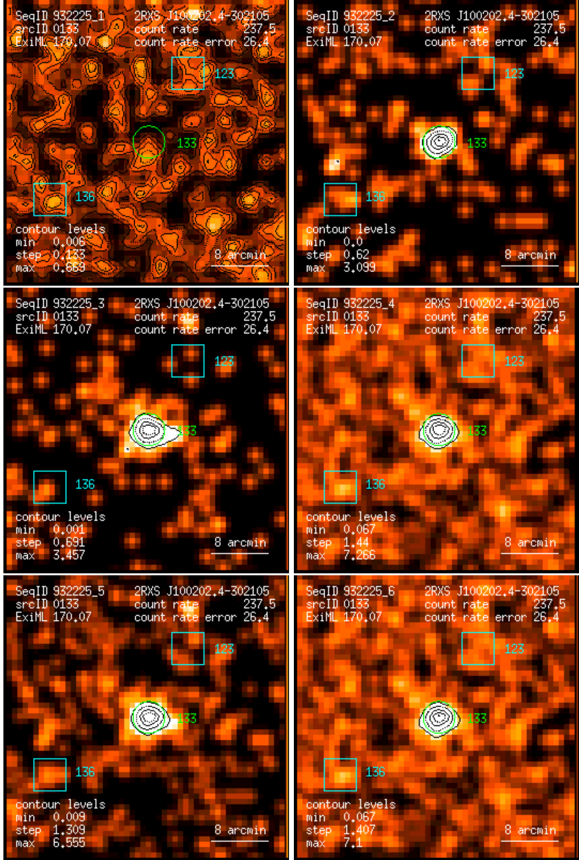
Figure 133: RASS 932225: detection 0133: band rate images, Gaussian filter: (1) PSPC channels 11 – 41, (2) 52 – 90, (3) 91 – 201, (4) 11 – 235, (5) 52 – 201, (6) 11 – 201. Broad band rates in counts/ks. Band rate contour levels in counts/ks/arcmin 2 .
