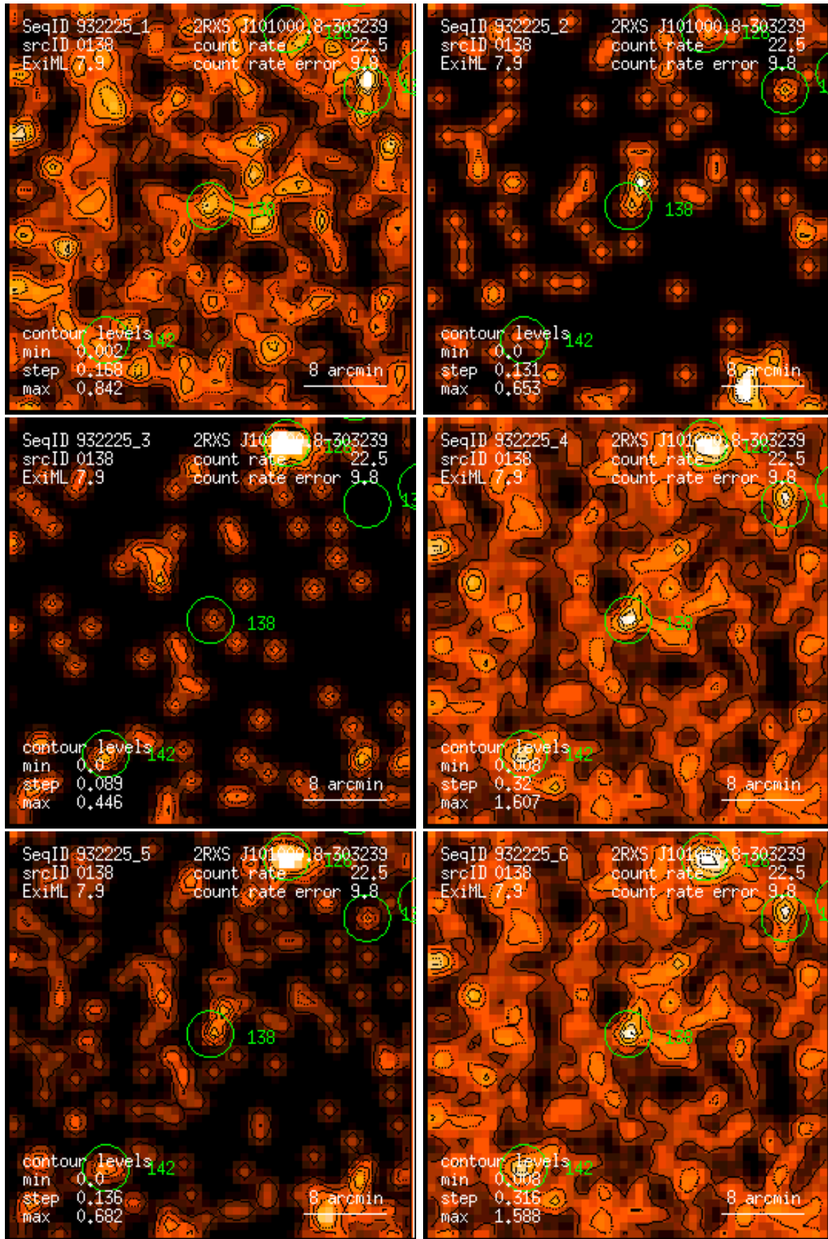
Figure 138: RASS 932225: detection 0138: band rate images, Gaussian filter: (1) PSPC channels 11 – 41, (2) 52 – 90, (3) 91 – 201, (4) 11 – 235, (5) 52 – 201, (6) 11 – 201. Broad band rates in counts/ks. Band rate contour levels in counts/ks/arcmin 2 .
