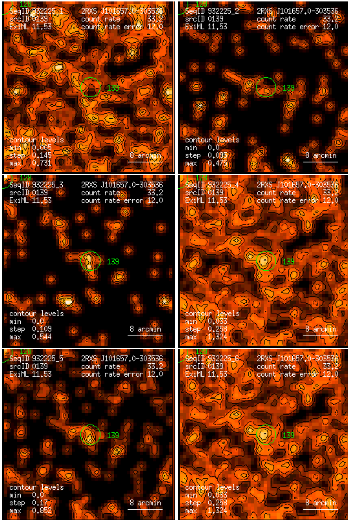
Figure 139: RASS 932225: detection 0139: band rate images, Gaussian filter: (1) PSPC channels 11 – 41, (2) 52 – 90, (3) 91 – 201, (4) 11 – 235, (5) 52 – 201, (6) 11 – 201. Broad band rates in counts/ks. Band rate contour levels in counts/ks/arcmin 2 .
