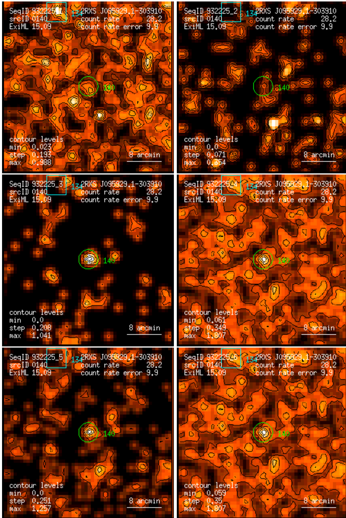
Figure 140: RASS 932225: detection 0140: band rate images, Gaussian filter: (1) PSPC channels 11 – 41, (2) 52 – 90, (3) 91 – 201, (4) 11 – 235, (5) 52 – 201, (6) 11 – 201. Broad band rates in counts/ks. Band rate contour levels in counts/ks/arcmin 2 .
