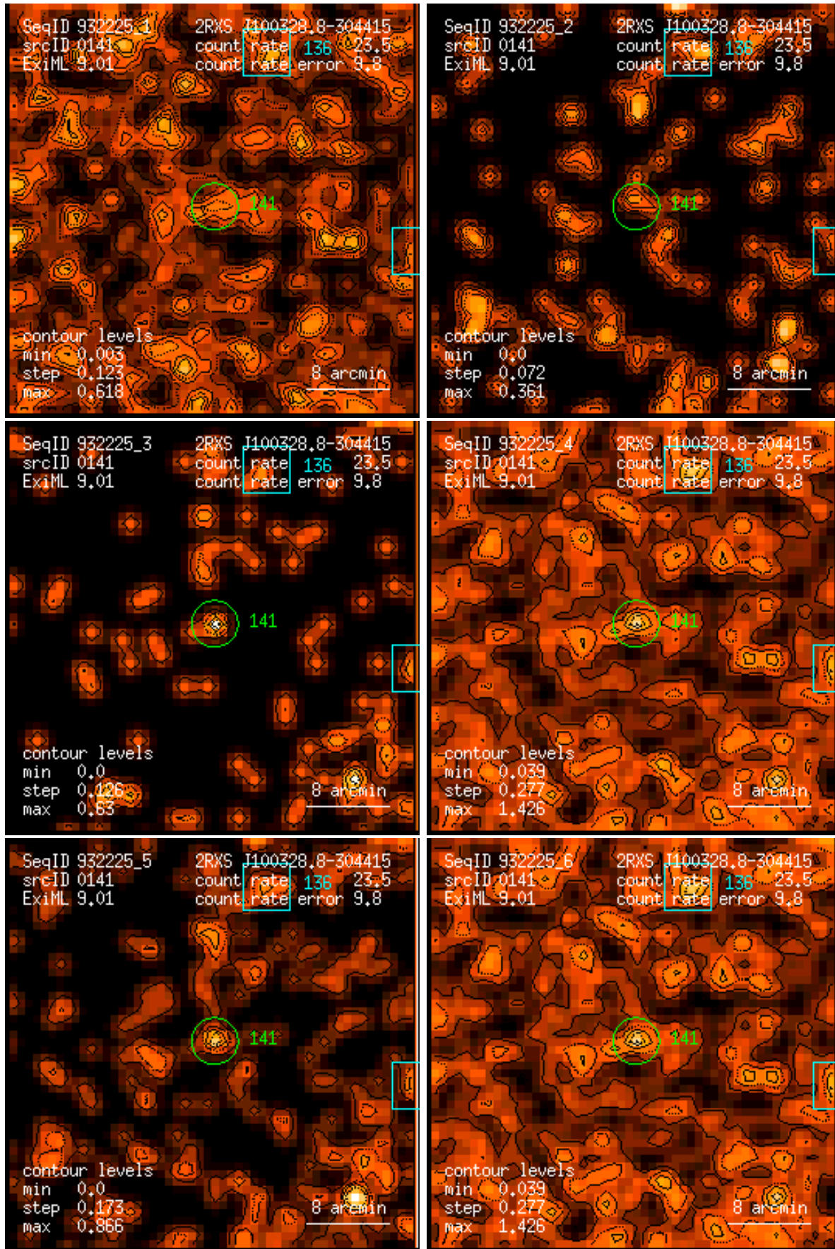
Figure 141: RASS 932225: detection 0141: band rate images, Gaussian filter: (1) PSPC channels 11 – 41, (2) 52 – 90, (3) 91 – 201, (4) 11 – 235, (5) 52 – 201, (6) 11 – 201. Broad band rates in counts/ks. Band rate contour levels in counts/ks/arcmin 2 .
