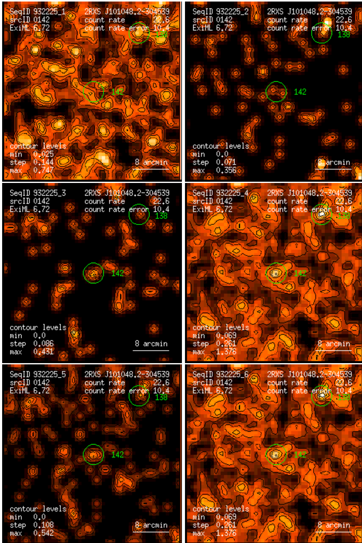
Figure 142: RASS 932225: detection 0142: band rate images, Gaussian filter: (1) PSPC channels 11 – 41, (2) 52 – 90, (3) 91 – 201, (4) 11 – 235, (5) 52 – 201, (6) 11 – 201. Broad band rates in counts/ks. Band rate contour levels in counts/ks/arcmin 2 .
