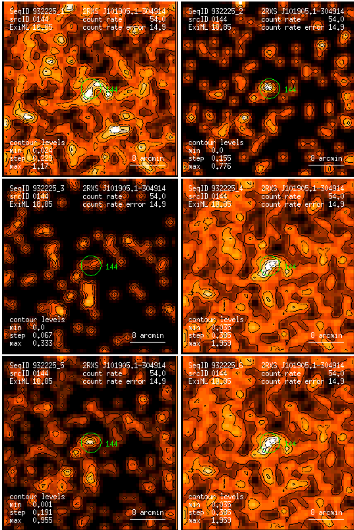
Figure 144: RASS 932225: detection 0144: band rate images, Gaussian filter: (1) PSPC channels 11 – 41, (2) 52 – 90, (3) 91 – 201, (4) 11 – 235, (5) 52 – 201, (6) 11 – 201. Broad band rates in counts/ks. Band rate contour levels in counts/ks/arcmin 2 .
