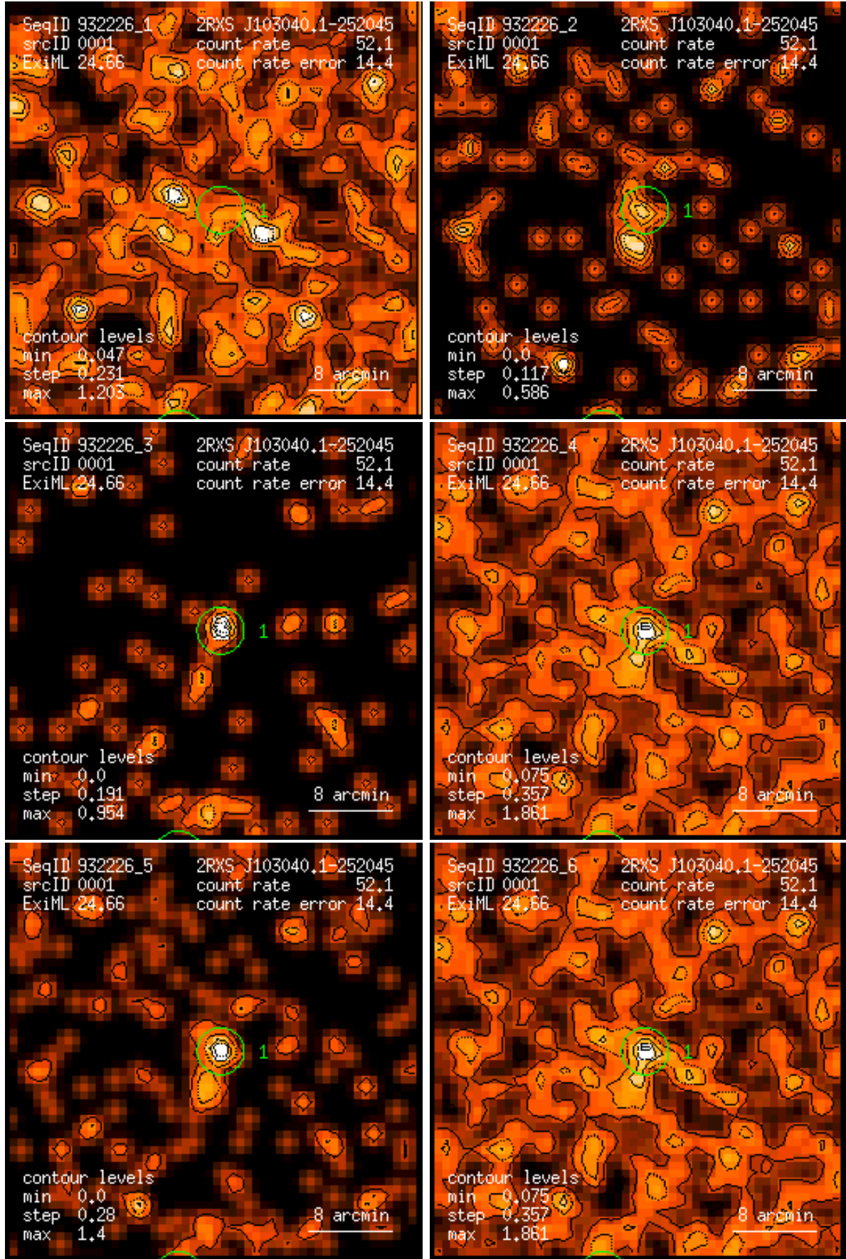
Figure 1: RASS 932226: detection 0001: band rate images, Gaussian filter: (1) PSPC channels 11 – 41, (2) 52 – 90, (3) 91 – 201, (4) 11 – 235, (5) 52 – 201, (6) 11 – 201. Broad band rates in counts/ks. Band rate contour levels in counts/ks/arcmin 2 .
