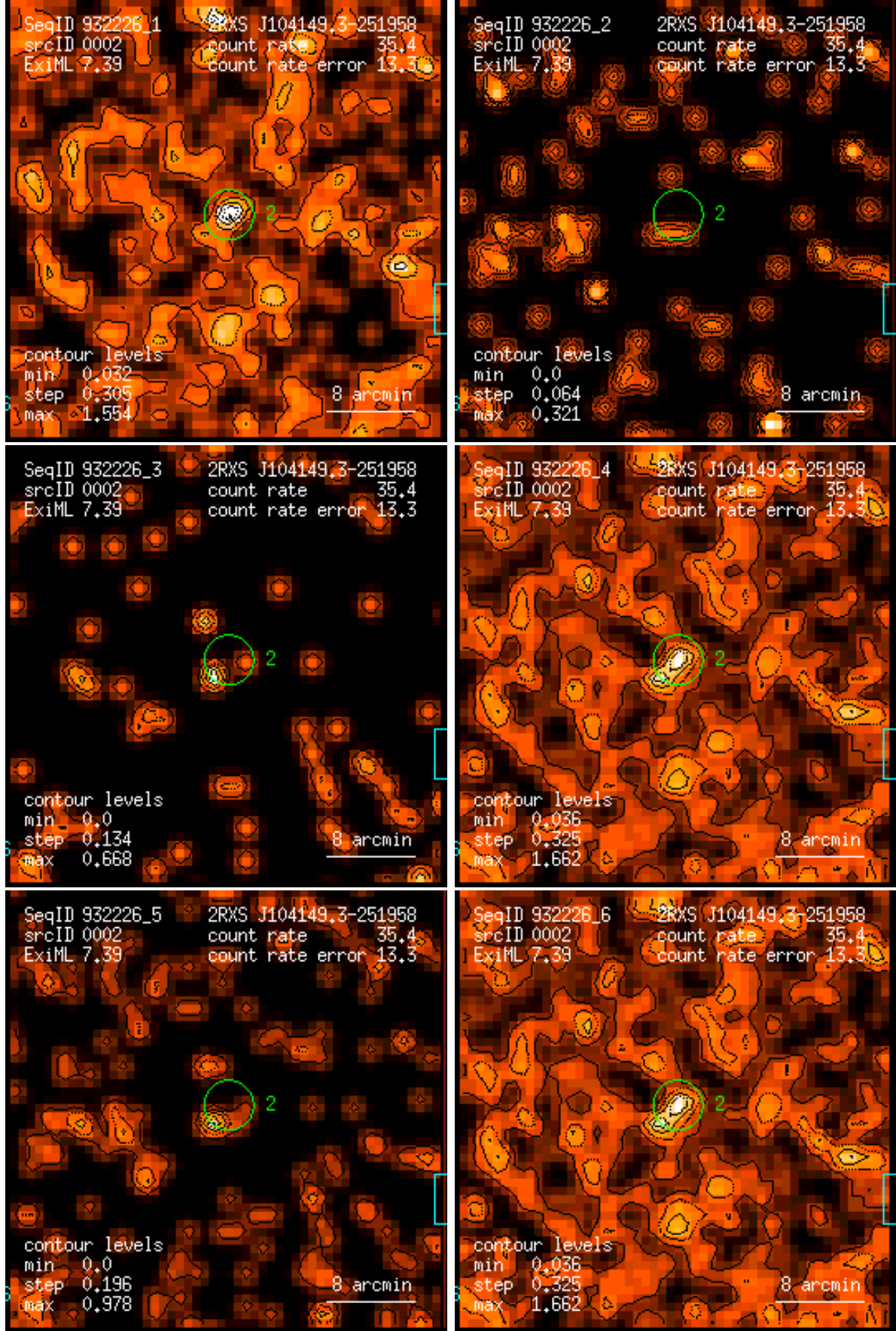
Figure 2: RASS 932226: detection 0002: band rate images, Gaussian filter: (1) PSPC channels 11 – 41, (2) 52 – 90, (3) 91 – 201, (4) 11 – 235, (5) 52 – 201, (6) 11 – 201. Broad band rates in counts/ks. Band rate contour levels in counts/ks/arcmin 2 .
