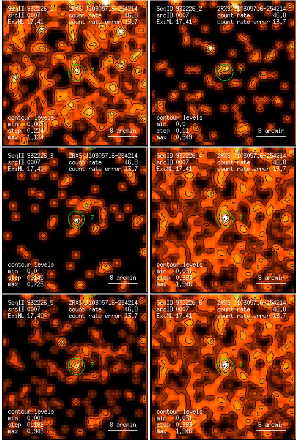
Figure 7: RASS 932226: detection 0007: band rate images, Gaussian filter: (1) PSPC channels 11 – 41, (2) 52 – 90, (3) 91 – 201, (4) 11 – 235, (5) 52 – 201, (6) 11 – 201. Broad band rates in counts/ks. Band rate contour levels in counts/ks/arcmin 2 .
