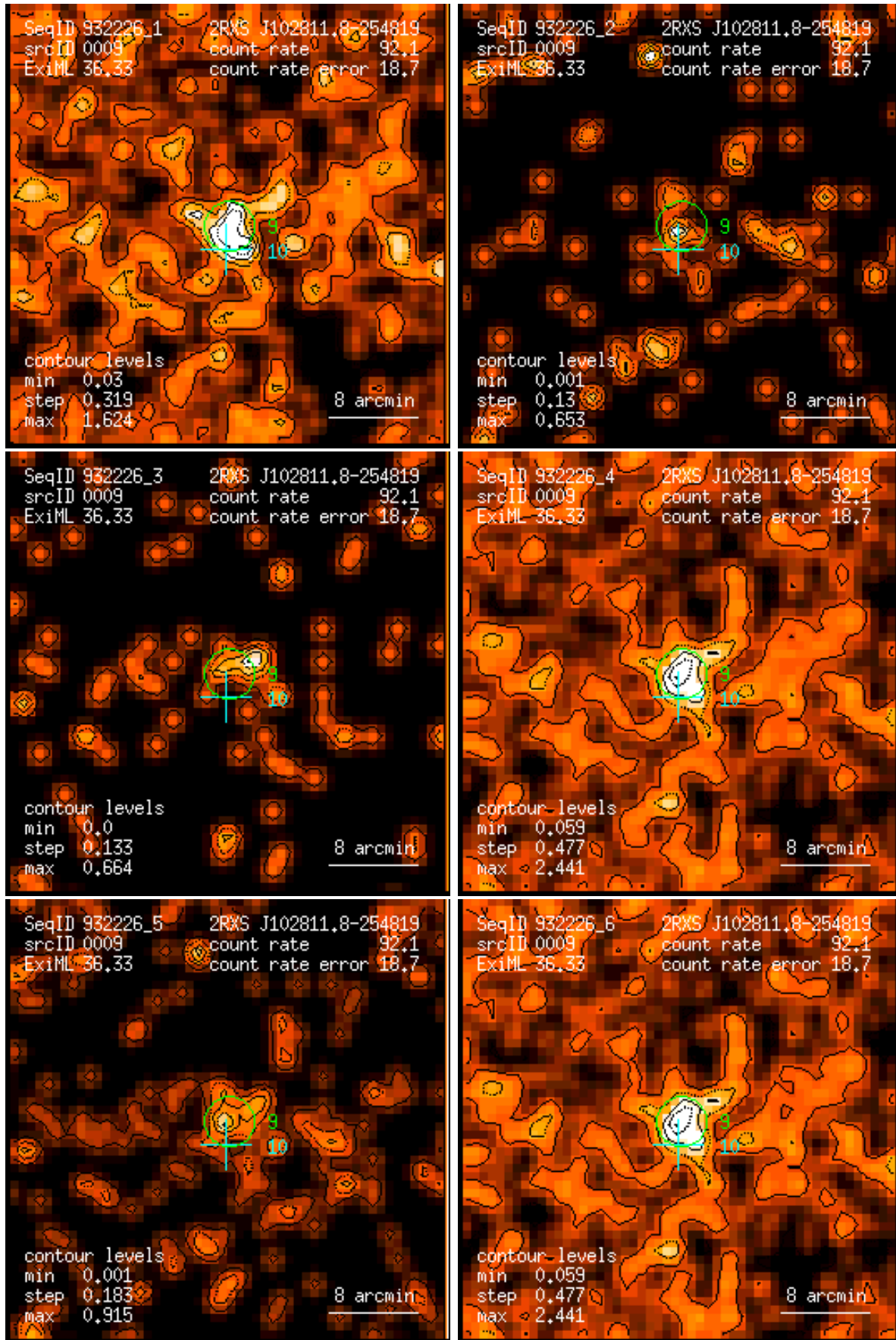
Figure 9: RASS 932226: detection 0009: band rate images, Gaussian filter: (1) PSPC channels 11 – 41, (2) 52 – 90, (3) 91 – 201, (4) 11 – 235, (5) 52 – 201, (6) 11 – 201. Broad band rates in counts/ks. Band rate contour levels in counts/ks/arcmin 2 .
