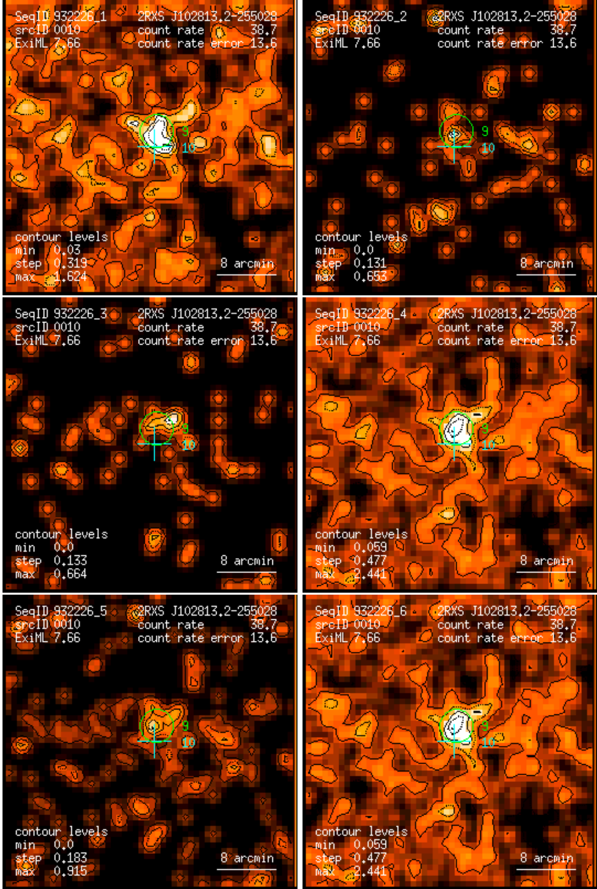
Figure 10: RASS 932226: detection 0010: band rate images, Gaussian filter: (1) PSPC channels 11 – 41, (2) 52 – 90, (3) 91 – 201, (4) 11 – 235, (5) 52 – 201, (6) 11 – 201. Broad band rates in counts/ks. Band rate contour levels in counts/ks/arcmin 2 .
