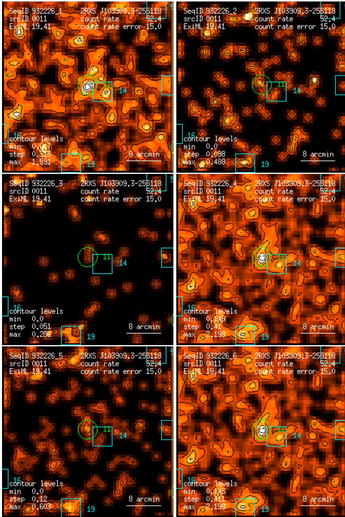
Figure 11: RASS 932226: detection 0011: band rate images, Gaussian filter: (1) PSPC channels 11 – 41, (2) 52 – 90, (3) 91 – 201, (4) 11 – 235, (5) 52 – 201, (6) 11 – 201. Broad band rates in counts/ks. Band rate contour levels in counts/ks/arcmin 2 .
