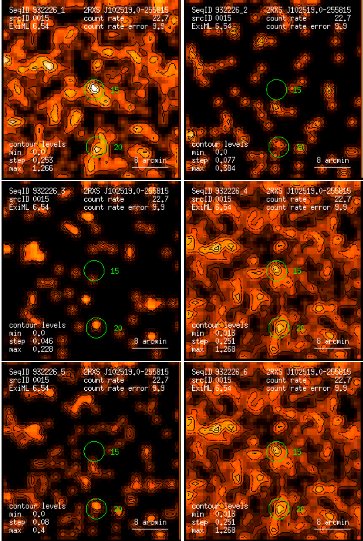
Figure 15: RASS 932226: detection 0015: band rate images, Gaussian filter: (1) PSPC channels 11 – 41, (2) 52 – 90, (3) 91 – 201, (4) 11 – 235, (5) 52 – 201, (6) 11 – 201. Broad band rates in counts/ks. Band rate contour levels in counts/ks/arcmin 2 .
