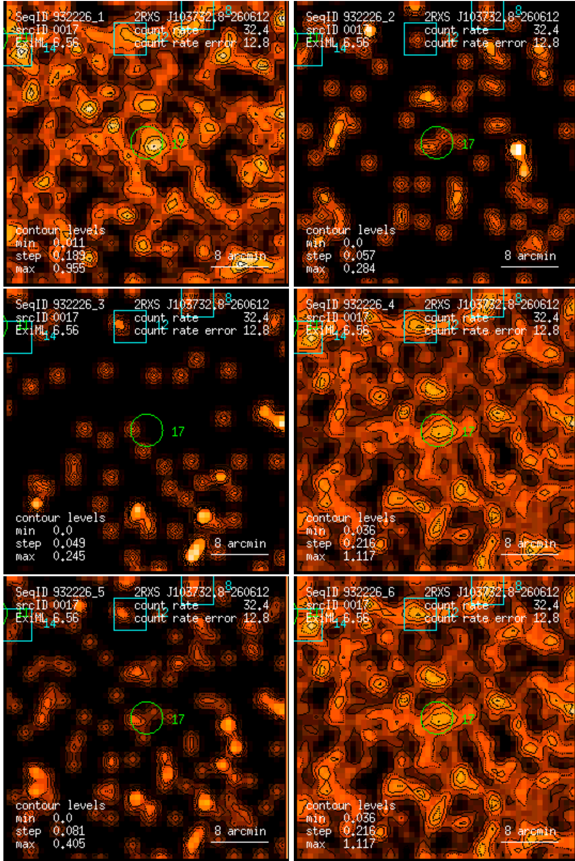
Figure 17: RASS 932226: detection 0017: band rate images, Gaussian filter: (1) PSPC channels 11 – 41, (2) 52 – 90, (3) 91 – 201, (4) 11 – 235, (5) 52 – 201, (6) 11 – 201. Broad band rates in counts/ks. Band rate contour levels in counts/ks/arcmin 2 .
