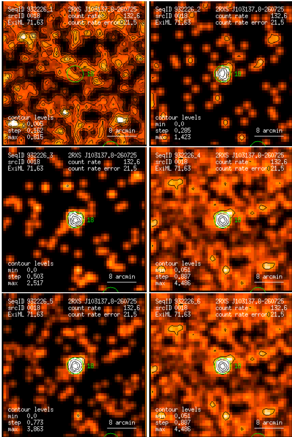
Figure 18: RASS 932226: detection 0018: band rate images, Gaussian filter: (1) PSPC channels 11 – 41, (2) 52 – 90, (3) 91 – 201, (4) 11 – 235, (5) 52 – 201, (6) 11 – 201. Broad band rates in counts/ks. Band rate contour levels in counts/ks/arcmin 2 .
