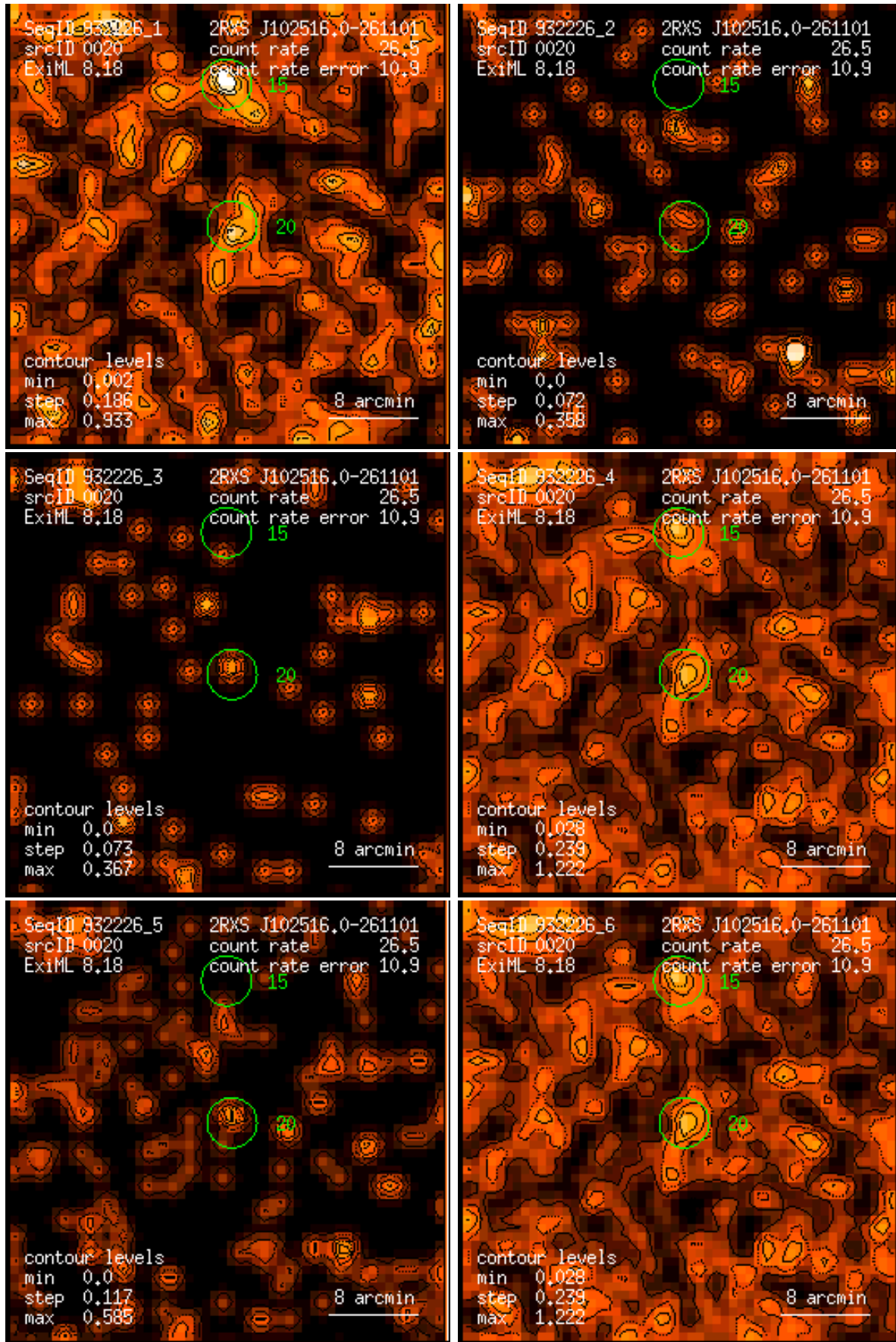
Figure 20: RASS 932226: detection 0020: band rate images, Gaussian filter: (1) PSPC channels 11 – 41, (2) 52 – 90, (3) 91 – 201, (4) 11 – 235, (5) 52 – 201, (6) 11 – 201. Broad band rates in counts/ks. Band rate contour levels in counts/ks/arcmin 2 .
