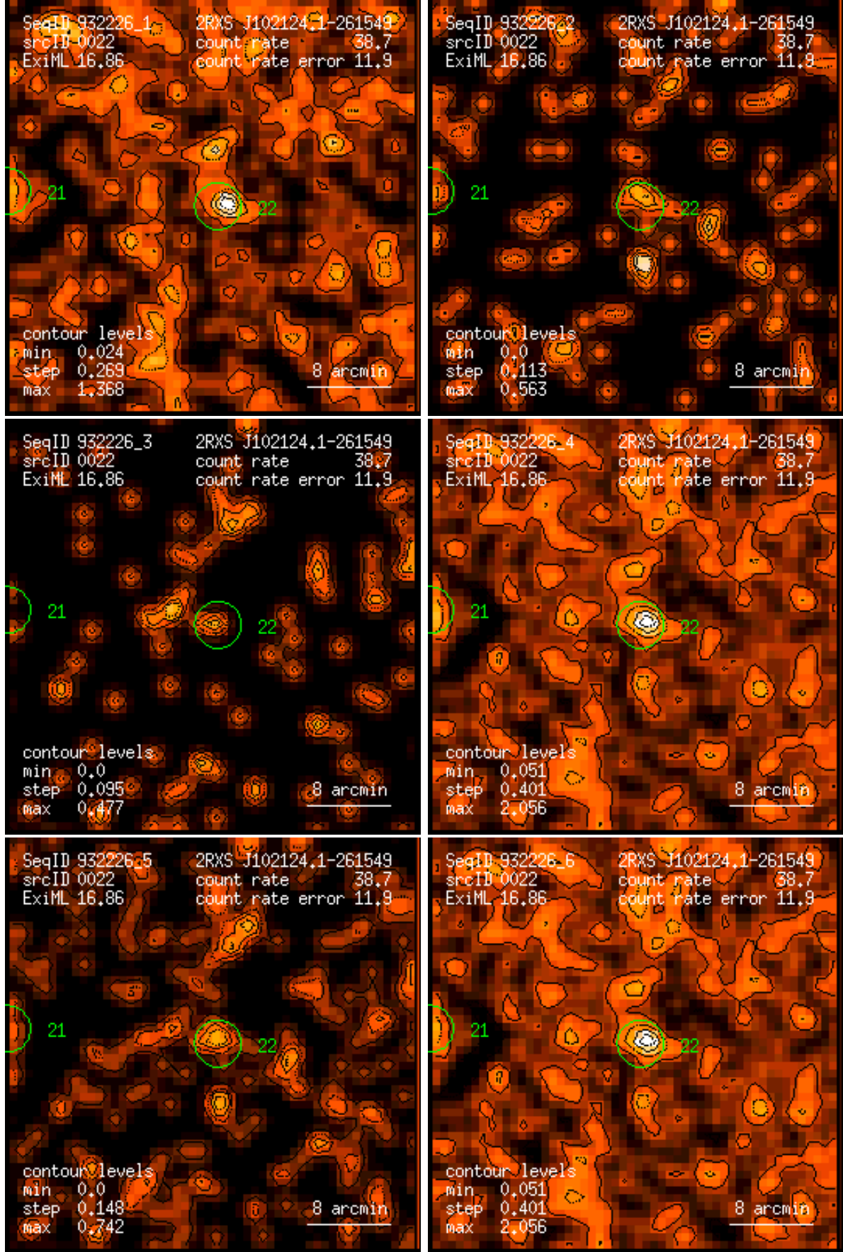
Figure 22: RASS 932226: detection 0022: band rate images, Gaussian filter: (1) PSPC channels 11 – 41, (2) 52 – 90, (3) 91 – 201, (4) 11 – 235, (5) 52 – 201, (6) 11 – 201. Broad band rates in counts/ks. Band rate contour levels in counts/ks/arcmin 2 .
