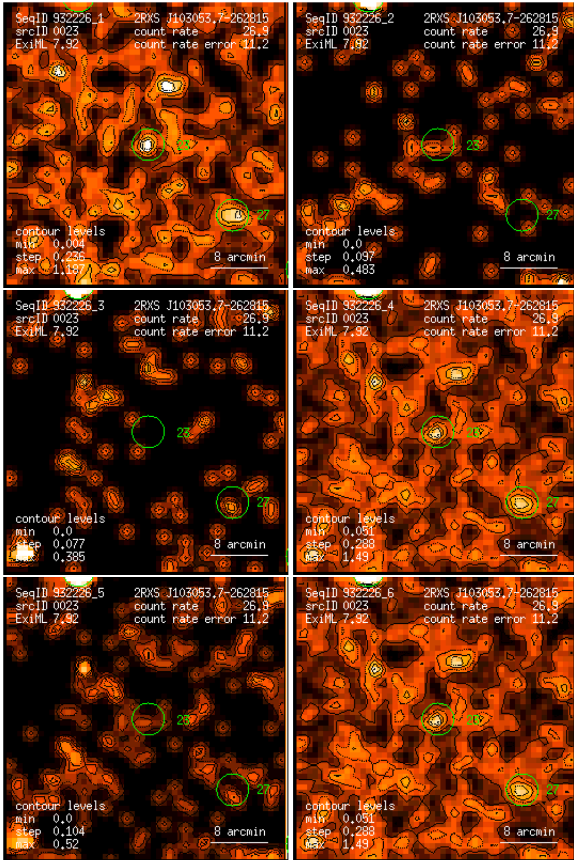
Figure 23: RASS 932226: detection 0023: band rate images, Gaussian filter: (1) PSPC channels 11 – 41, (2) 52 – 90, (3) 91 – 201, (4) 11 – 235, (5) 52 – 201, (6) 11 – 201. Broad band rates in counts/ks. Band rate contour levels in counts/ks/arcmin 2 .
