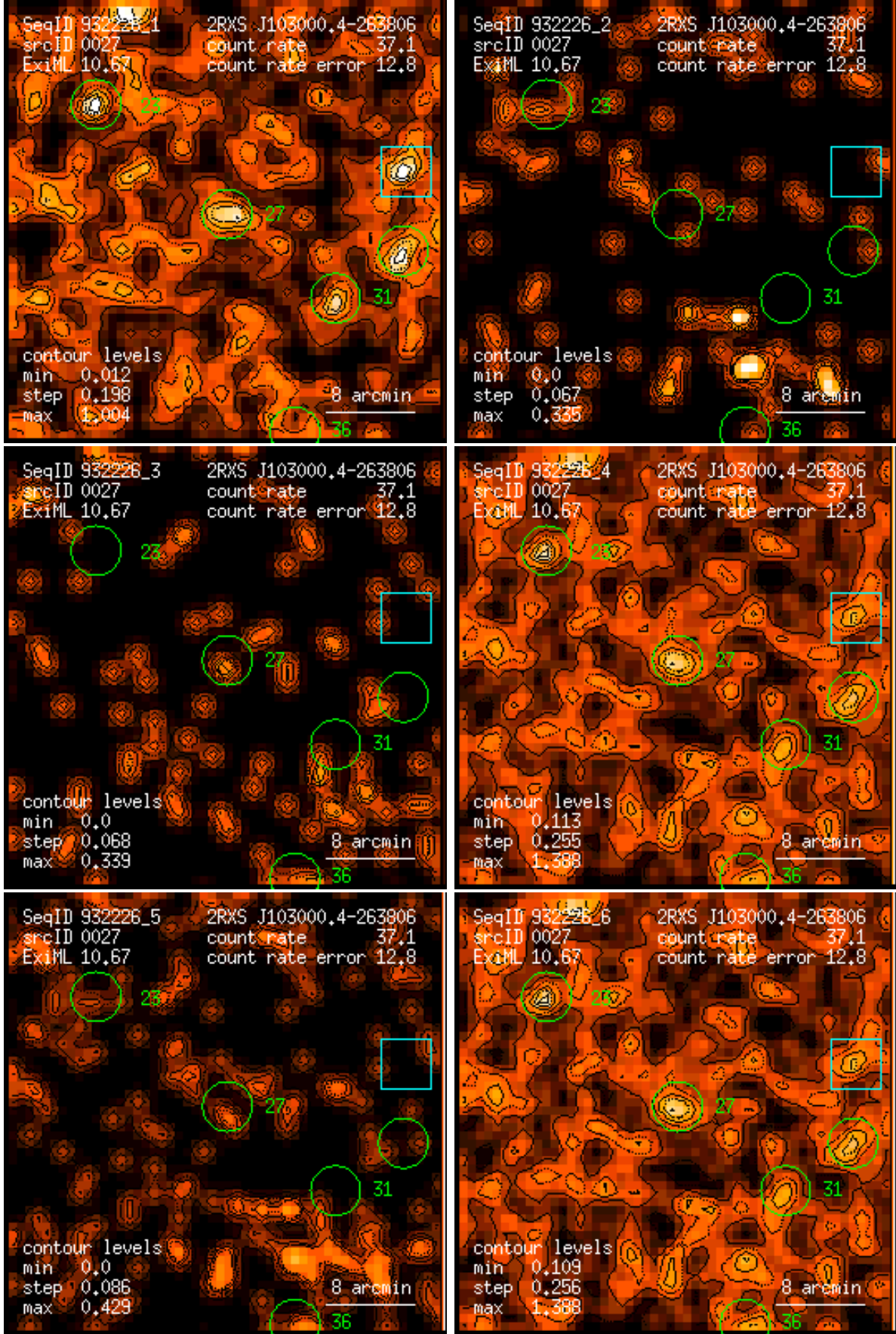
Figure 27: RASS 932226: detection 0027: band rate images, Gaussian filter: (1) PSPC channels 11 – 41, (2) 52 – 90, (3) 91 – 201, (4) 11 – 235, (5) 52 – 201, (6) 11 – 201. Broad band rates in counts/ks. Band rate contour levels in counts/ks/arcmin 2 .
