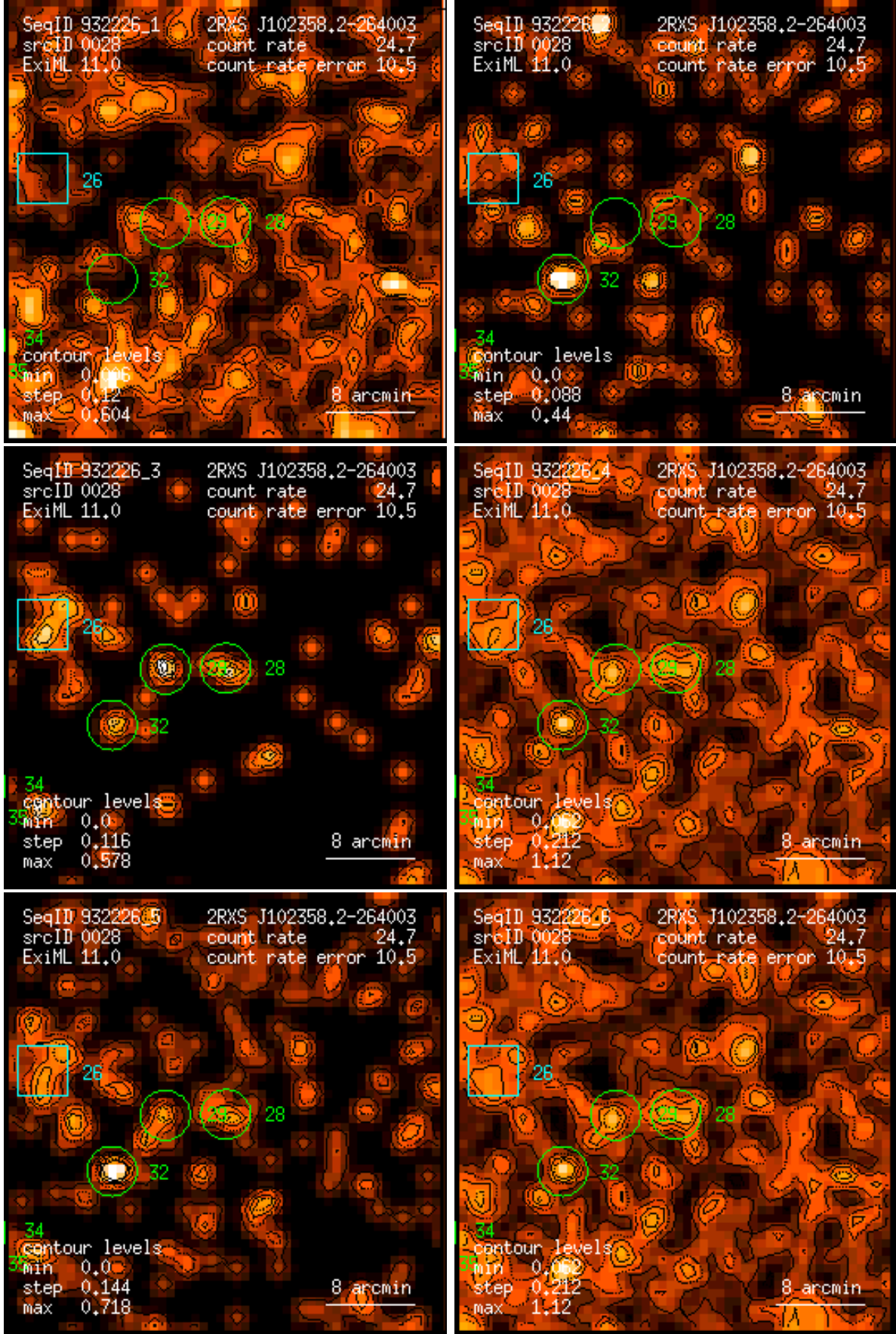
Figure 28: RASS 932226: detection 0028: band rate images, Gaussian filter: (1) PSPC channels 11 – 41, (2) 52 – 90, (3) 91 – 201, (4) 11 – 235, (5) 52 – 201, (6) 11 – 201. Broad band rates in counts/ks. Band rate contour levels in counts/ks/arcmin 2 .
