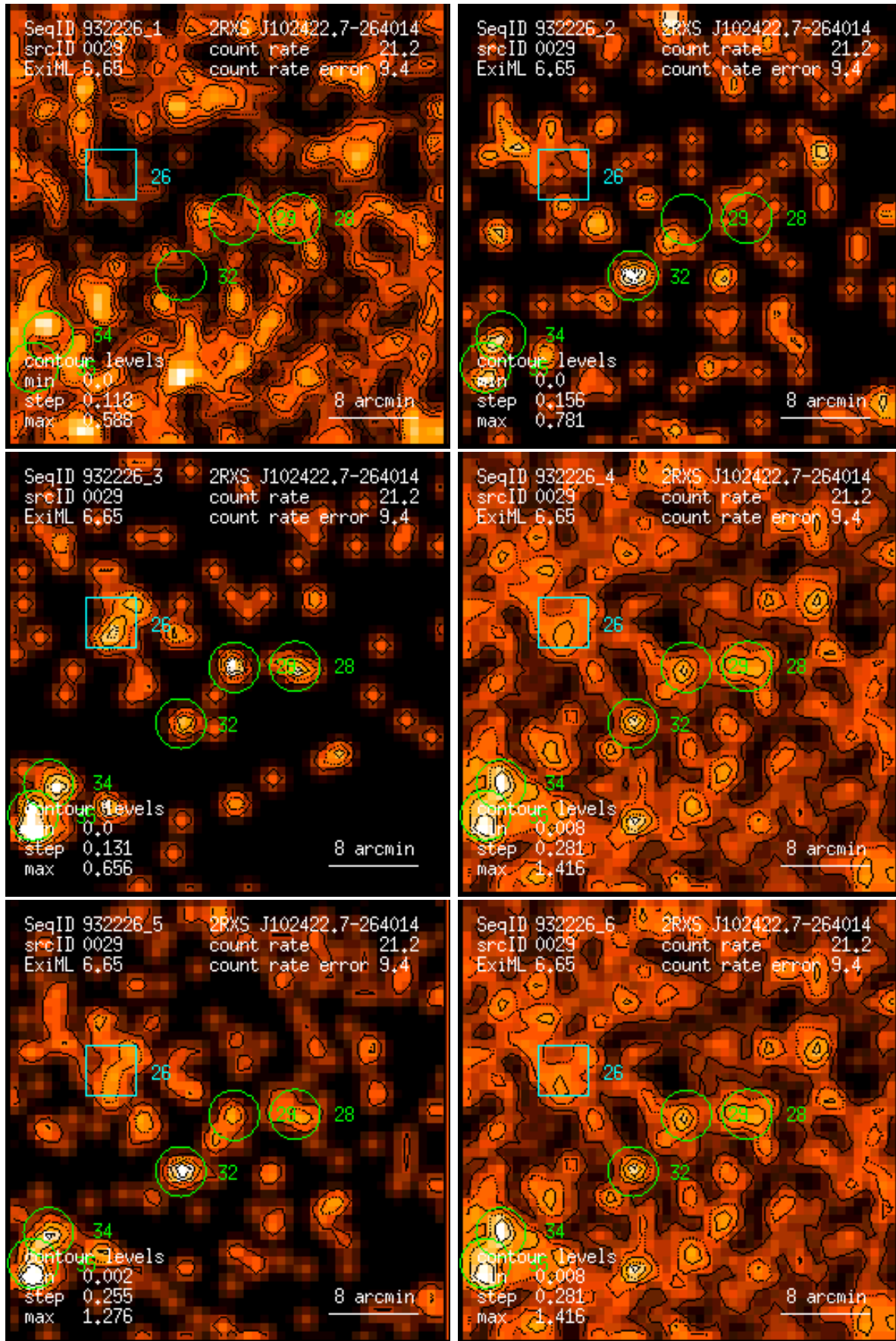
Figure 29: RASS 932226: detection 0029: band rate images, Gaussian filter: (1) PSPC channels 11 – 41, (2) 52 – 90, (3) 91 – 201, (4) 11 – 235, (5) 52 – 201, (6) 11 – 201. Broad band rates in counts/ks. Band rate contour levels in counts/ks/arcmin 2 .
