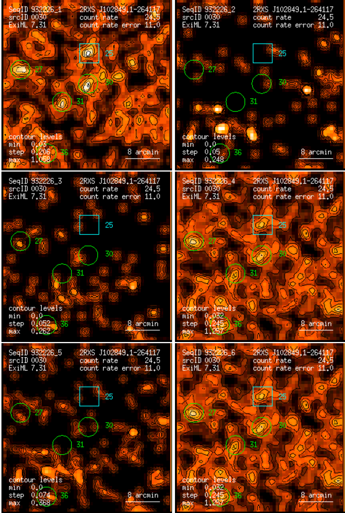
Figure 30: RASS 932226: detection 0030: band rate images, Gaussian filter: (1) PSPC channels 11 – 41, (2) 52 – 90, (3) 91 – 201, (4) 11 – 235, (5) 52 – 201, (6) 11 – 201. Broad band rates in counts/ks. Band rate contour levels in counts/ks/arcmin 2 .
