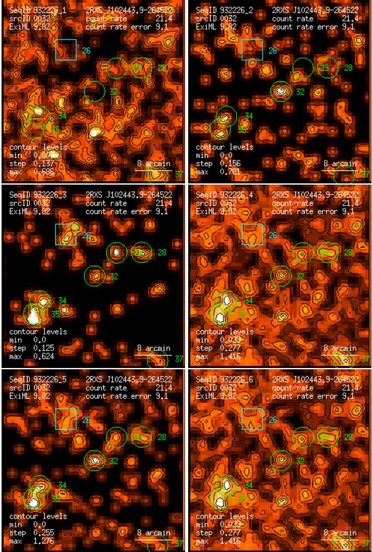
Figure 32: RASS 932226: detection 0032: band rate images, Gaussian filter: (1) PSPC channels 11 – 41, (2) 52 – 90, (3) 91 – 201, (4) 11 – 235, (5) 52 – 201, (6) 11 – 201. Broad band rates in counts/ks. Band rate contour levels in counts/ks/arcmin 2 .
