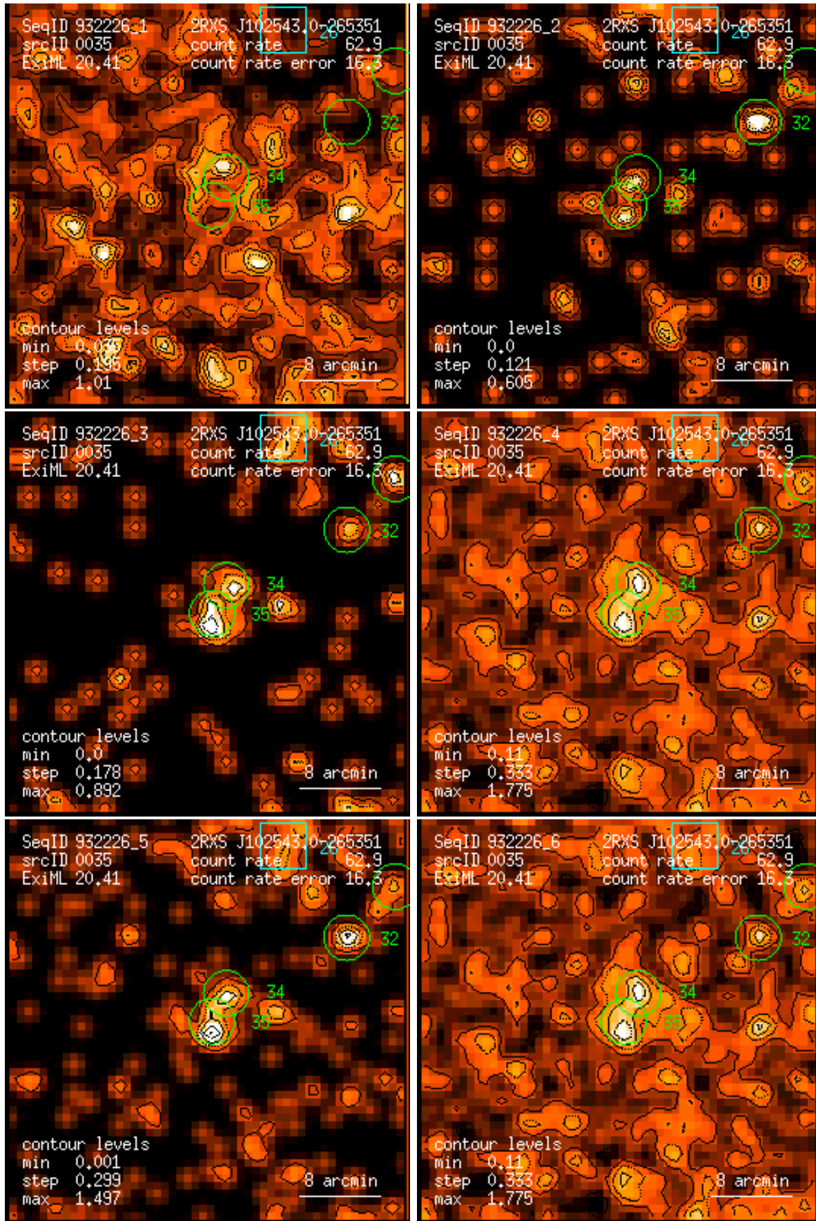
Figure 35: RASS 932226: detection 0035: band rate images, Gaussian filter: (1) PSPC channels 11 – 41, (2) 52 – 90, (3) 91 – 201, (4) 11 – 235, (5) 52 – 201, (6) 11 – 201. Broad band rates in counts/ks. Band rate contour levels in counts/ks/arcmin 2 .
