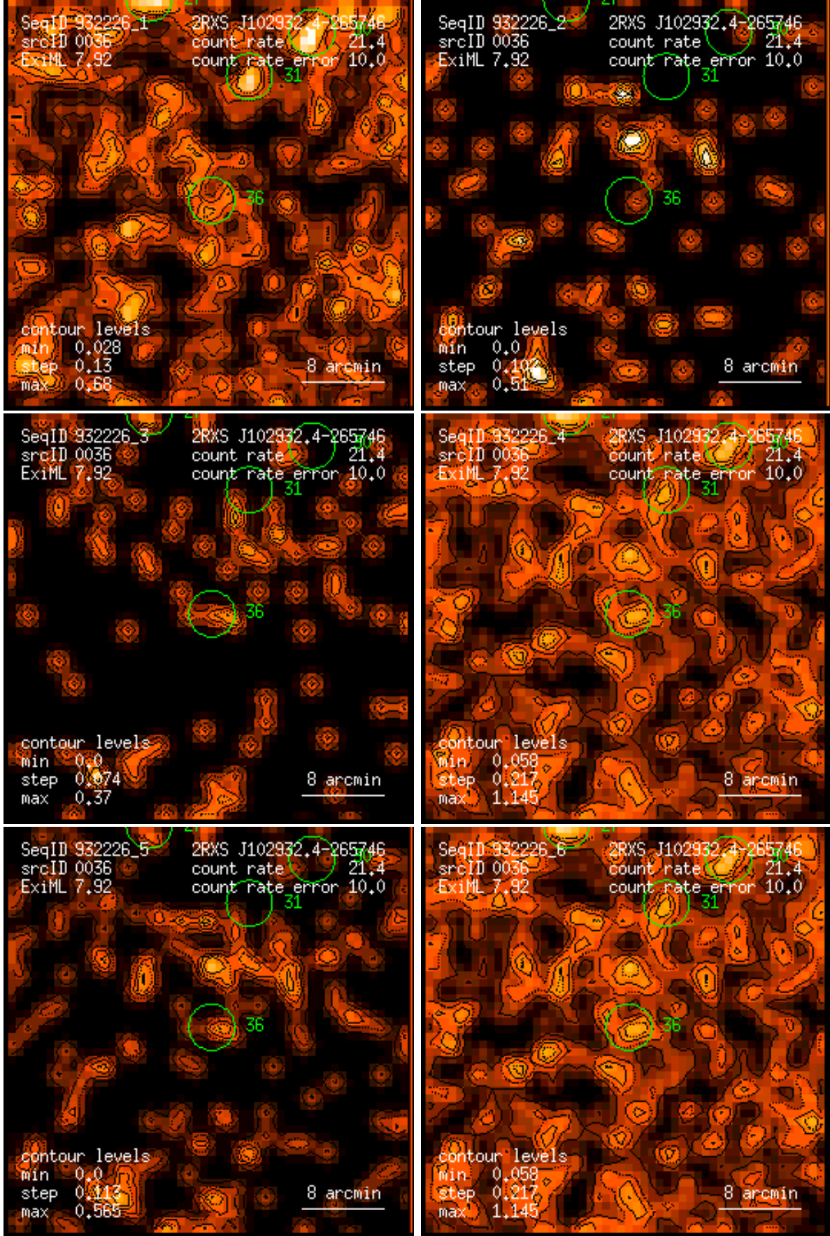
Figure 36: RASS 932226: detection 0036: band rate images, Gaussian filter: (1) PSPC channels 11 – 41, (2) 52 – 90, (3) 91 – 201, (4) 11 – 235, (5) 52 – 201, (6) 11 – 201. Broad band rates in counts/ks. Band rate contour levels in counts/ks/arcmin 2 .
