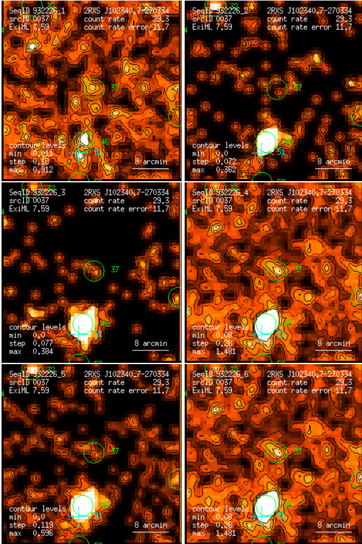
Figure 37: RASS 932226: detection 0037: band rate images, Gaussian filter: (1) PSPC channels 11 – 41, (2) 52 – 90, (3) 91 – 201, (4) 11 – 235, (5) 52 – 201, (6) 11 – 201. Broad band rates in counts/ks. Band rate contour levels in counts/ks/arcmin 2 .
