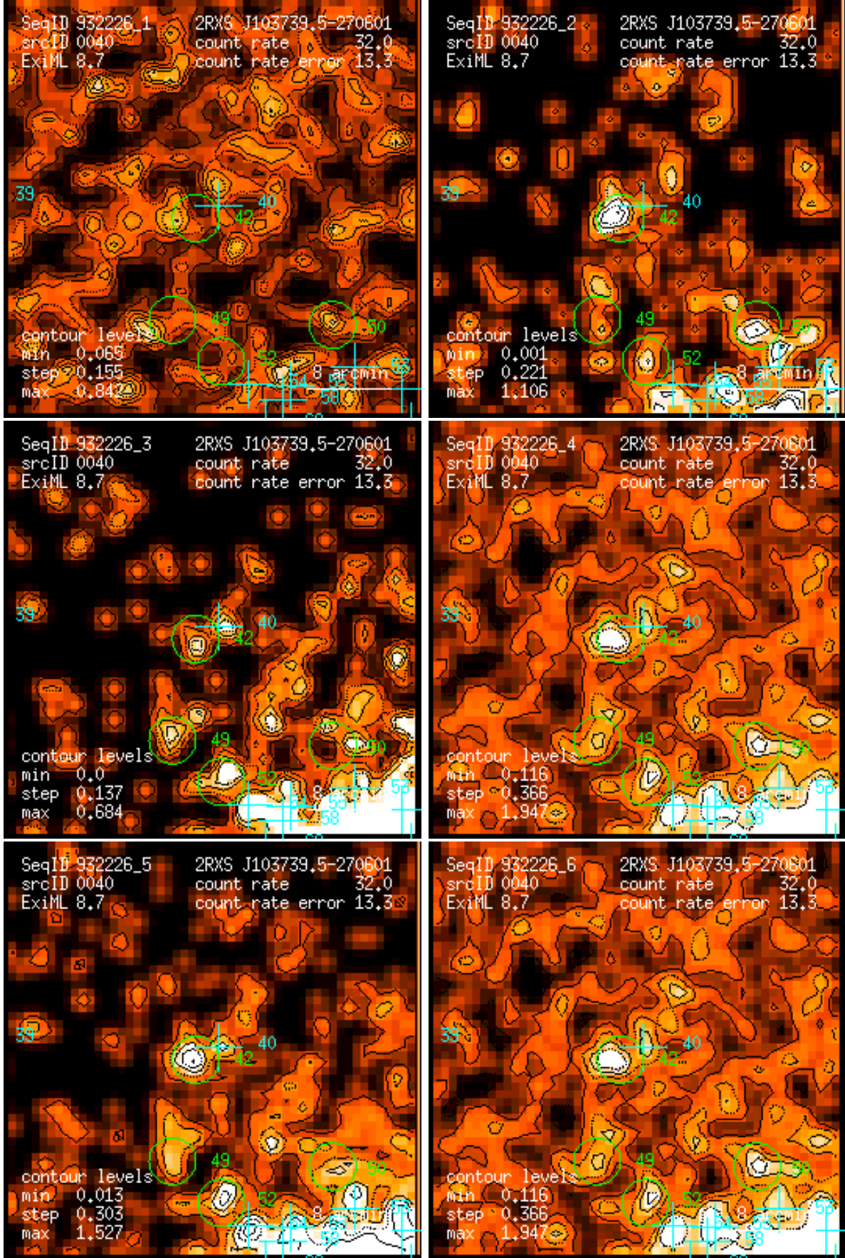
Figure 40: RASS 932226: detection 0040: band rate images, Gaussian filter: (1) PSPC channels 11 – 41, (2) 52 – 90, (3) 91 – 201, (4) 11 – 235, (5) 52 – 201, (6) 11 – 201. Broad band rates in counts/ks. Band rate contour levels in counts/ks/arcmin 2 .
