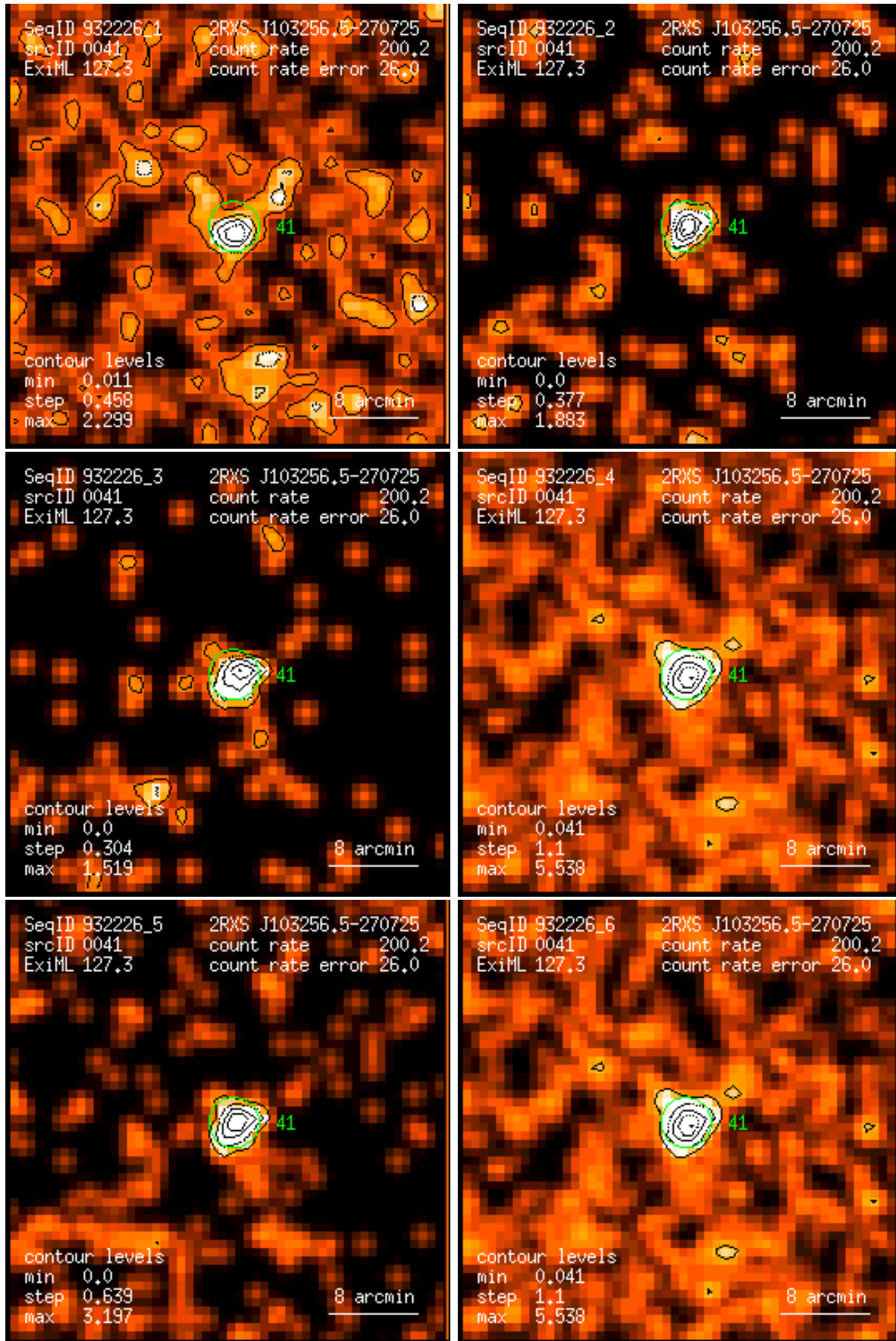
Figure 41: RASS 932226: detection 0041: band rate images, Gaussian filter: (1) PSPC channels 11 – 41, (2) 52 – 90, (3) 91 – 201, (4) 11 – 235, (5) 52 – 201, (6) 11 – 201. Broad band rates in counts/ks. Band rate contour levels in counts/ks/arcmin 2 .
