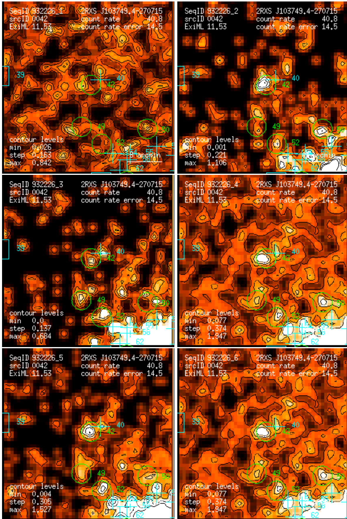
Figure 42: RASS 932226: detection 0042: band rate images, Gaussian filter: (1) PSPC channels 11 – 41, (2) 52 – 90, (3) 91 – 201, (4) 11 – 235, (5) 52 – 201, (6) 11 – 201. Broad band rates in counts/ks. Band rate contour levels in counts/ks/arcmin 2 .
