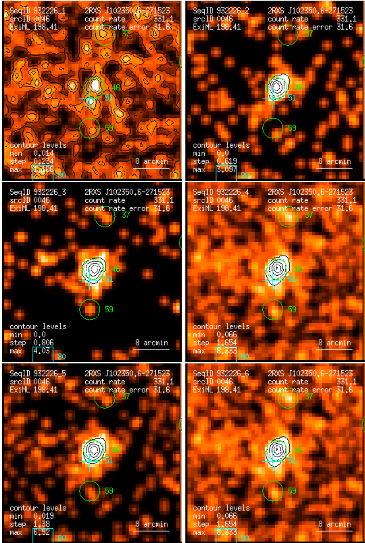
Figure 46: RASS 932226: detection 0046: band rate images, Gaussian filter: (1) PSPC channels 11 – 41, (2) 52 – 90, (3) 91 – 201, (4) 11 – 235, (5) 52 – 201, (6) 11 – 201. Broad band rates in counts/ks. Band rate contour levels in counts/ks/arcmin 2 .
