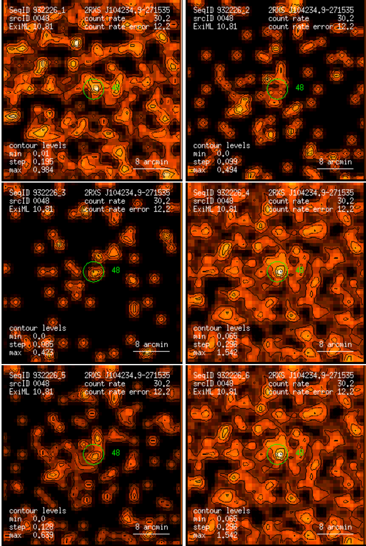
Figure 48: RASS 932226: detection 0048: band rate images, Gaussian filter: (1) PSPC channels 11 – 41, (2) 52 – 90, (3) 91 – 201, (4) 11 – 235, (5) 52 – 201, (6) 11 – 201. Broad band rates in counts/ks. Band rate contour levels in counts/ks/arcmin 2 .
