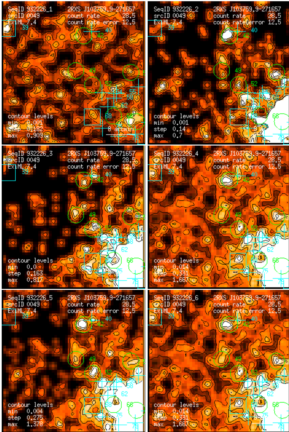
Figure 49: RASS 932226: detection 0049: band rate images, Gaussian filter: (1) PSPC channels 11 – 41, (2) 52 – 90, (3) 91 – 201, (4) 11 – 235, (5) 52 – 201, (6) 11 – 201. Broad band rates in counts/ks. Band rate contour levels in counts/ks/arcmin 2 .
