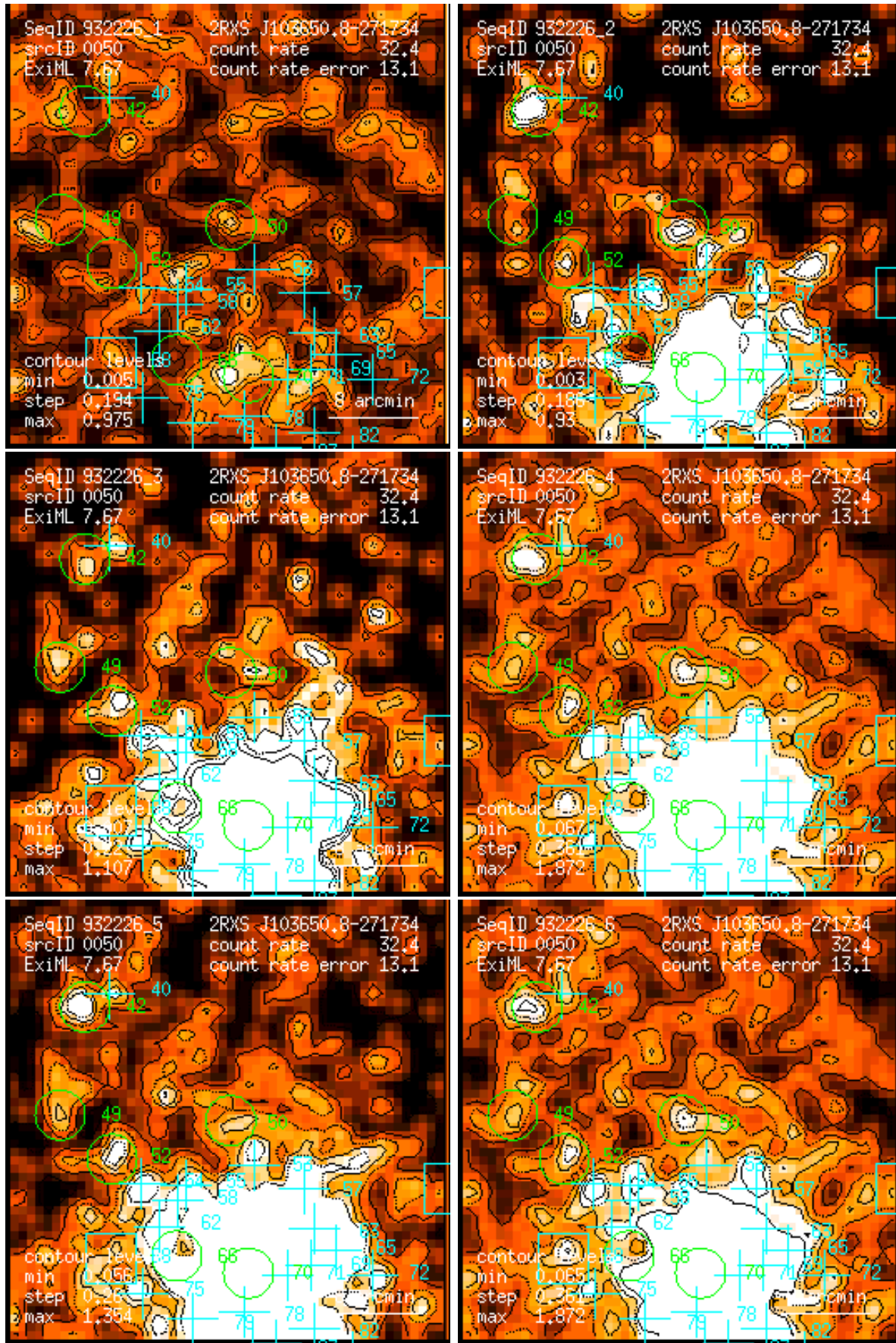
Figure 50: RASS 932226: detection 0050: band rate images, Gaussian filter: (1) PSPC channels 11 – 41, (2) 52 – 90, (3) 91 – 201, (4) 11 – 235, (5) 52 – 201, (6) 11 – 201. Broad band rates in counts/ks. Band rate contour levels in counts/ks/arcmin 2 .
