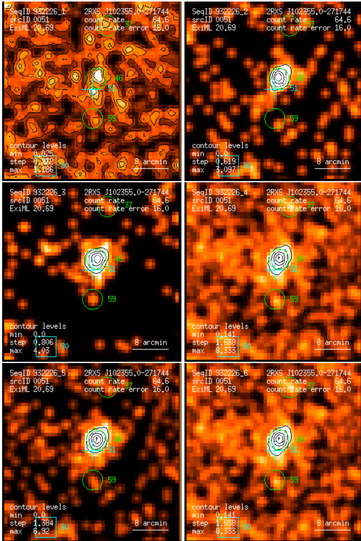
Figure 51: RASS 932226: detection 0051: band rate images, Gaussian filter: (1) PSPC channels 11 – 41, (2) 52 – 90, (3) 91 – 201, (4) 11 – 235, (5) 52 – 201, (6) 11 – 201. Broad band rates in counts/ks. Band rate contour levels in counts/ks/arcmin 2 .
