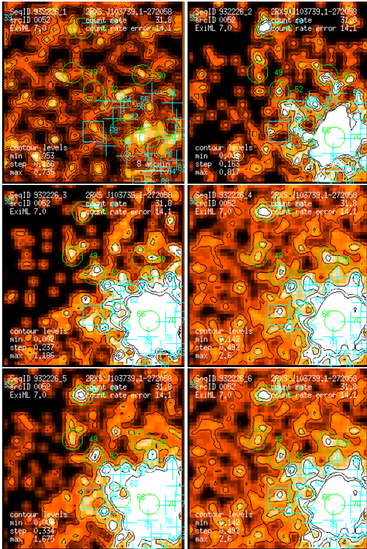
Figure 52: RASS 932226: detection 0052: band rate images, Gaussian filter: (1) PSPC channels 11 – 41, (2) 52 – 90, (3) 91 – 201, (4) 11 – 235, (5) 52 – 201, (6) 11 – 201. Broad band rates in counts/ks. Band rate contour levels in counts/ks/arcmin 2 .
