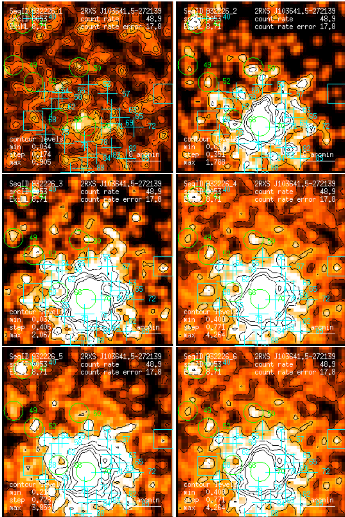
Figure 53: RASS 932226: detection 0053: band rate images, Gaussian filter: (1) PSPC channels 11 – 41, (2) 52 – 90, (3) 91 – 201, (4) 11 – 235, (5) 52 – 201, (6) 11 – 201. Broad band rates in counts/ks. Band rate contour levels in counts/ks/arcmin 2 .
