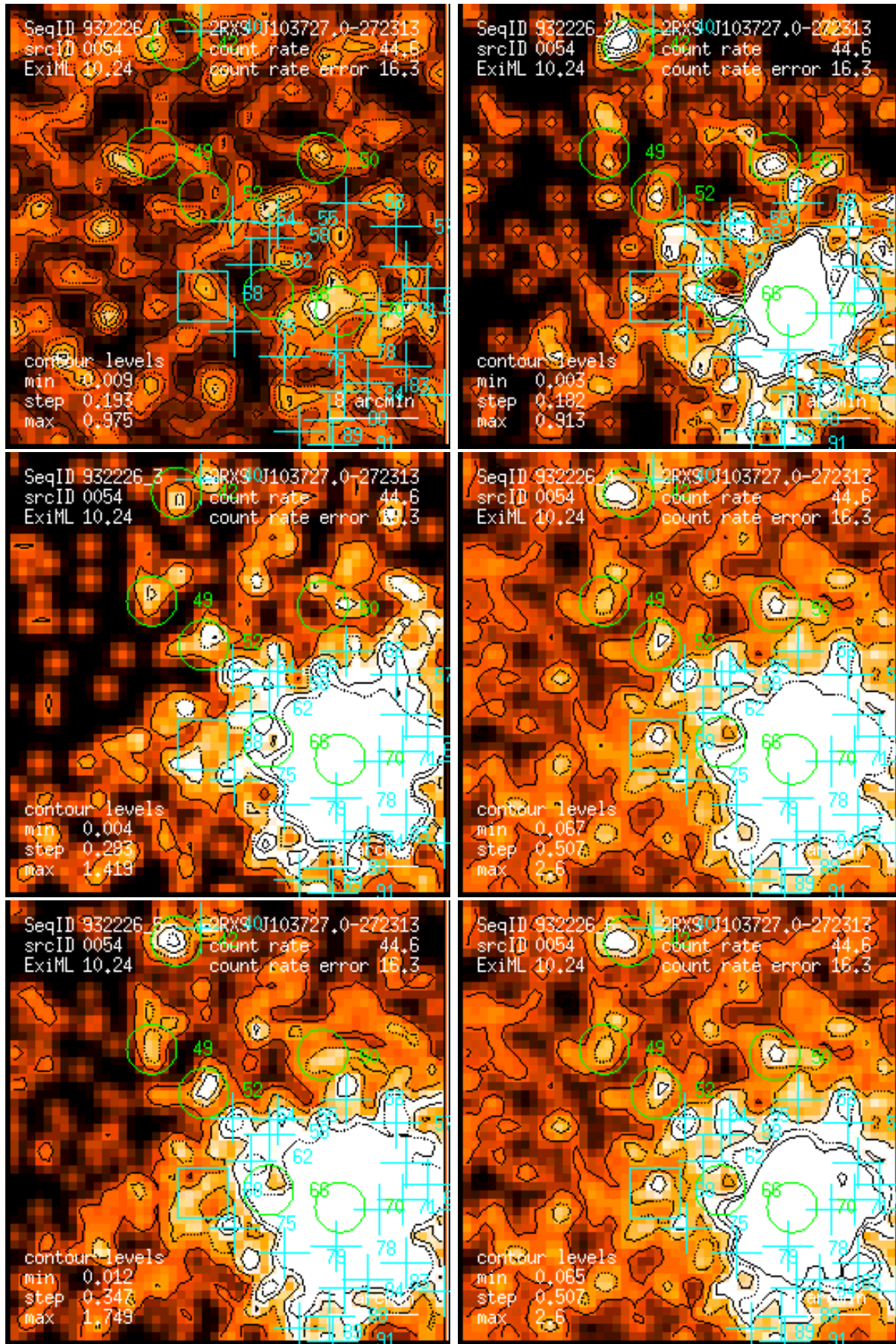
Figure 54: RASS 932226: detection 0054: band rate images, Gaussian filter: (1) PSPC channels 11 – 41, (2) 52 – 90, (3) 91 – 201, (4) 11 – 235, (5) 52 – 201, (6) 11 – 201. Broad band rates in counts/ks. Band rate contour levels in counts/ks/arcmin 2 .
