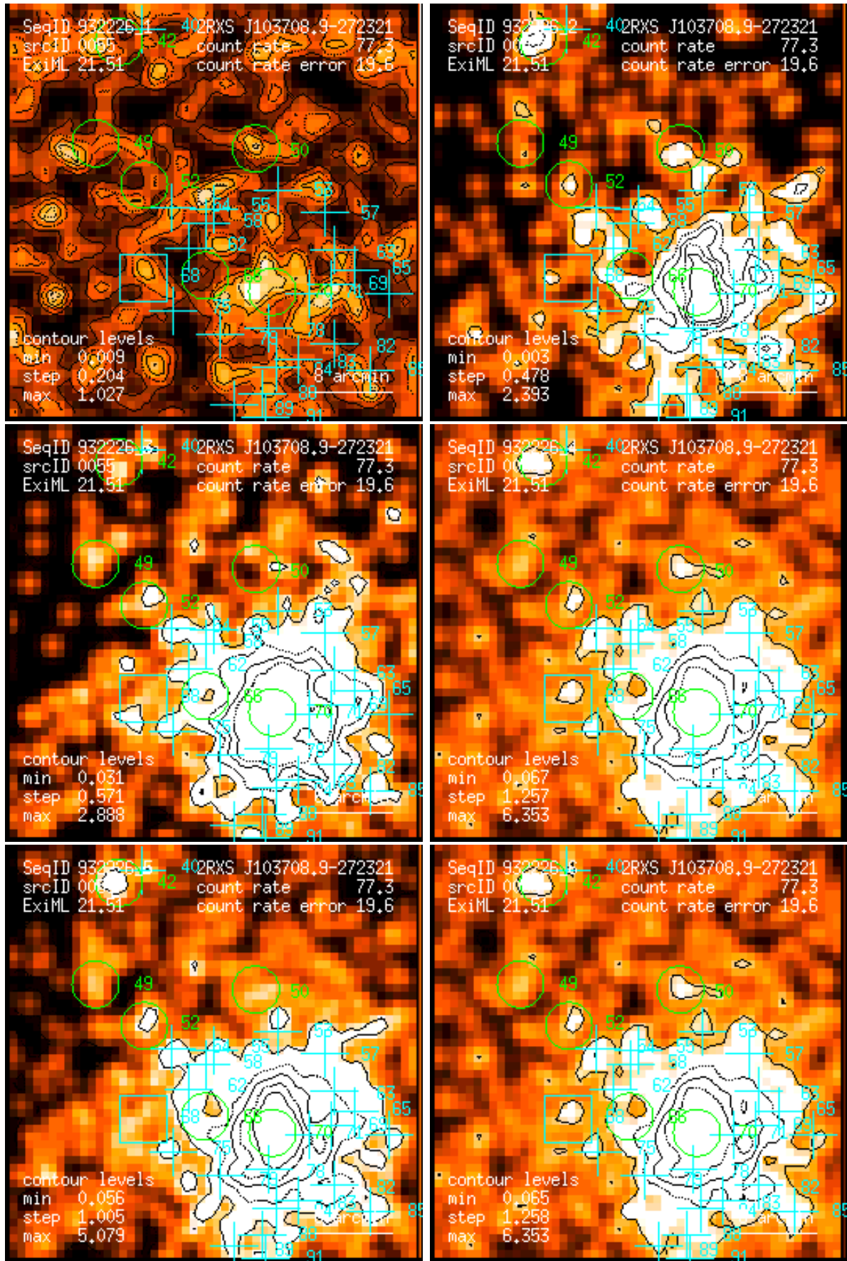
Figure 55: RASS 932226: detection 0055: band rate images, Gaussian filter: (1) PSPC channels 11 – 41, (2) 52 – 90, (3) 91 – 201, (4) 11 – 235, (5) 52 – 201, (6) 11 – 201. Broad band rates in counts/ks. Band rate contour levels in counts/ks/arcmin 2 .
