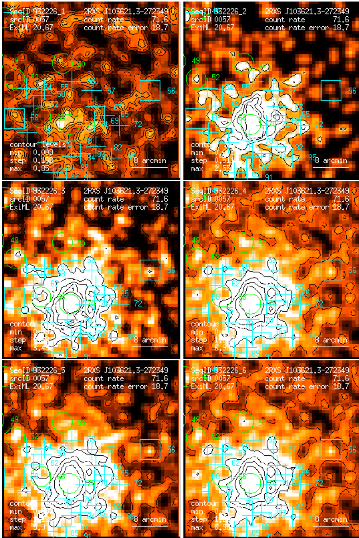
Figure 57: RASS 932226: detection 0057: band rate images, Gaussian filter: (1) PSPC channels 11 – 41, (2) 52 – 90, (3) 91 – 201, (4) 11 – 235, (5) 52 – 201, (6) 11 – 201. Broad band rates in counts/ks. Band rate contour levels in counts/ks/arcmin 2 .
