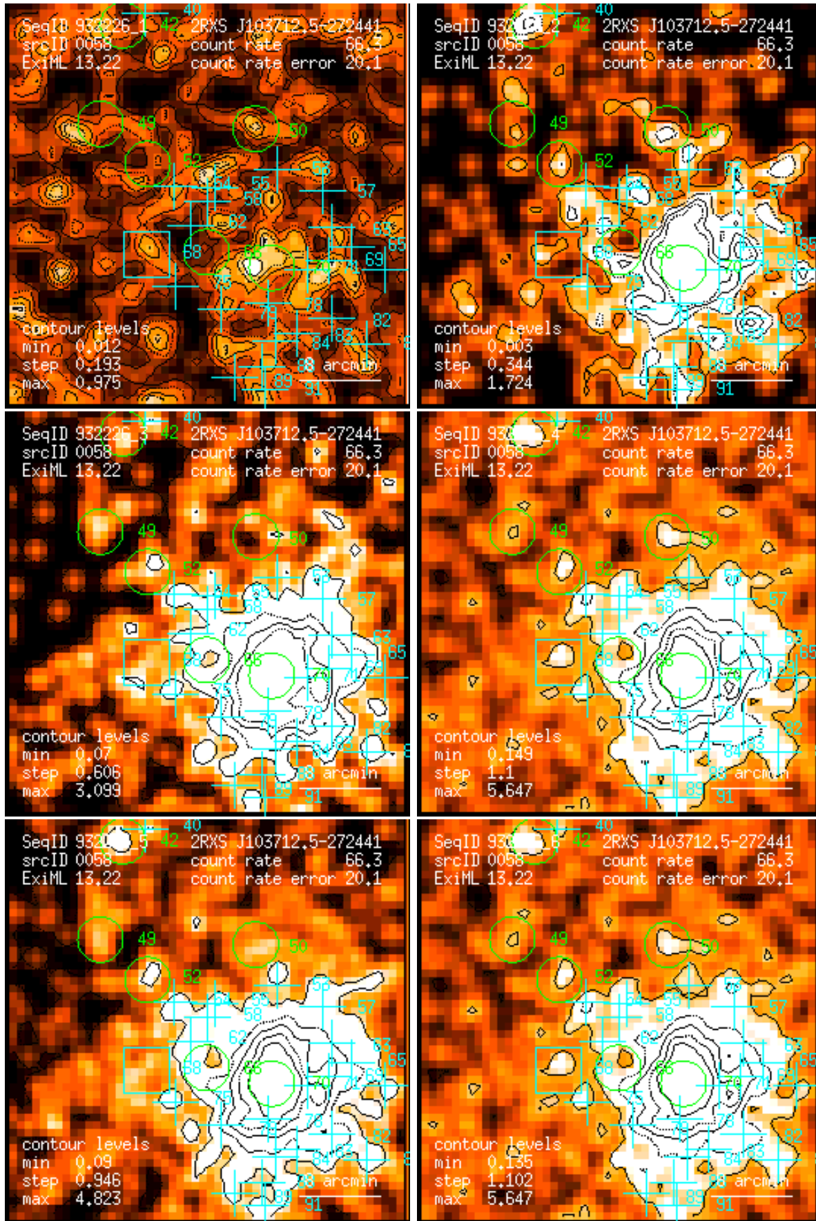
Figure 58: RASS 932226: detection 0058: band rate images, Gaussian filter: (1) PSPC channels 11 – 41, (2) 52 – 90, (3) 91 – 201, (4) 11 – 235, (5) 52 – 201, (6) 11 – 201. Broad band rates in counts/ks. Band rate contour levels in counts/ks/arcmin 2 .
