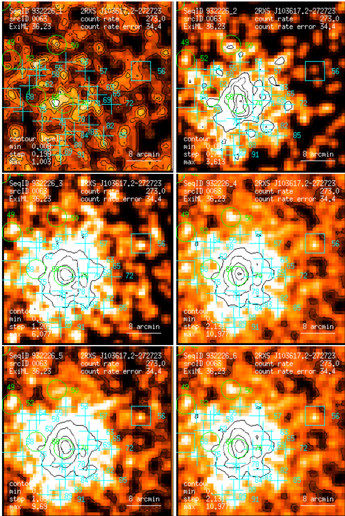
Figure 63: RASS 932226: detection 0063: band rate images, Gaussian filter: (1) PSPC channels 11 – 41, (2) 52 – 90, (3) 91 – 201, (4) 11 – 235, (5) 52 – 201, (6) 11 – 201. Broad band rates in counts/ks. Band rate contour levels in counts/ks/arcmin 2 .
