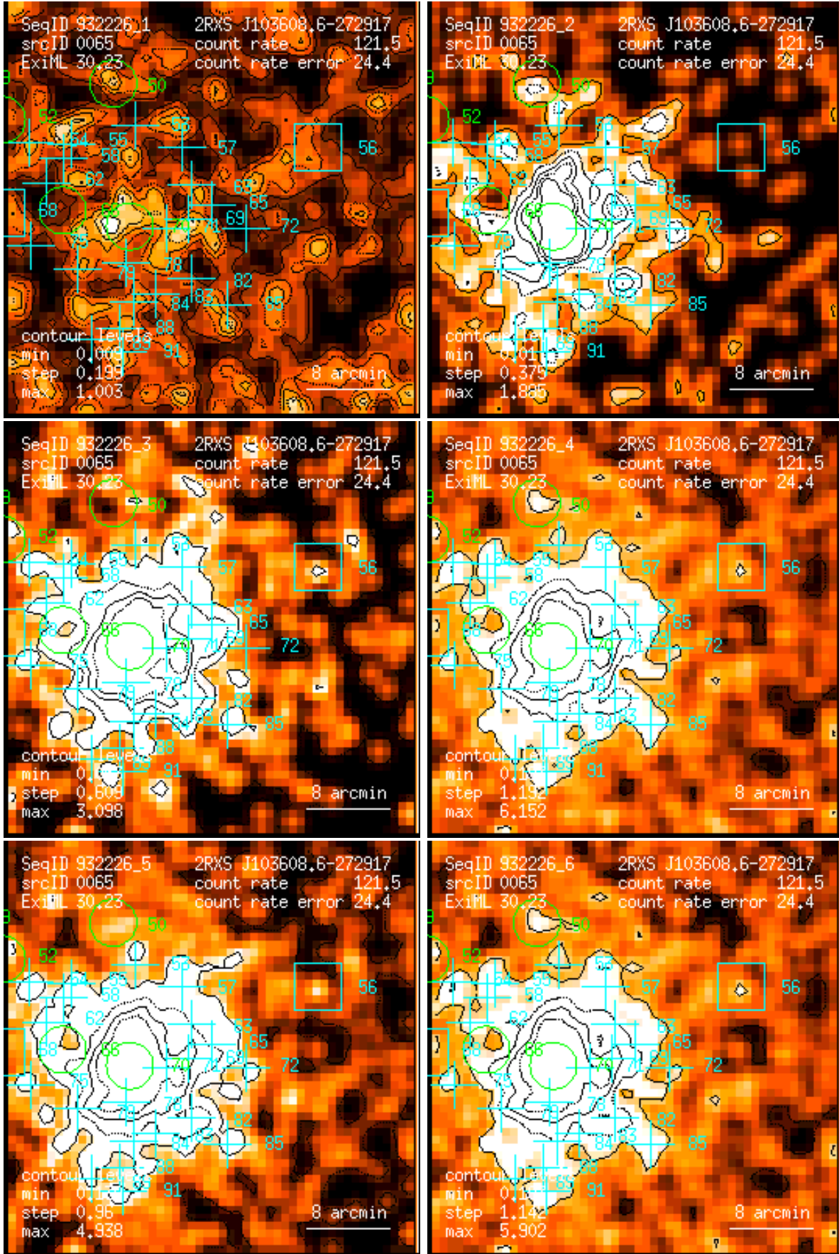
Figure 65: RASS 932226: detection 0065: band rate images, Gaussian filter: (1) PSPC channels 11 – 41, (2) 52 – 90, (3) 91 – 201, (4) 11 – 235, (5) 52 – 201, (6) 11 – 201. Broad band rates in counts/ks. Band rate contour levels in counts/ks/arcmin 2 .
