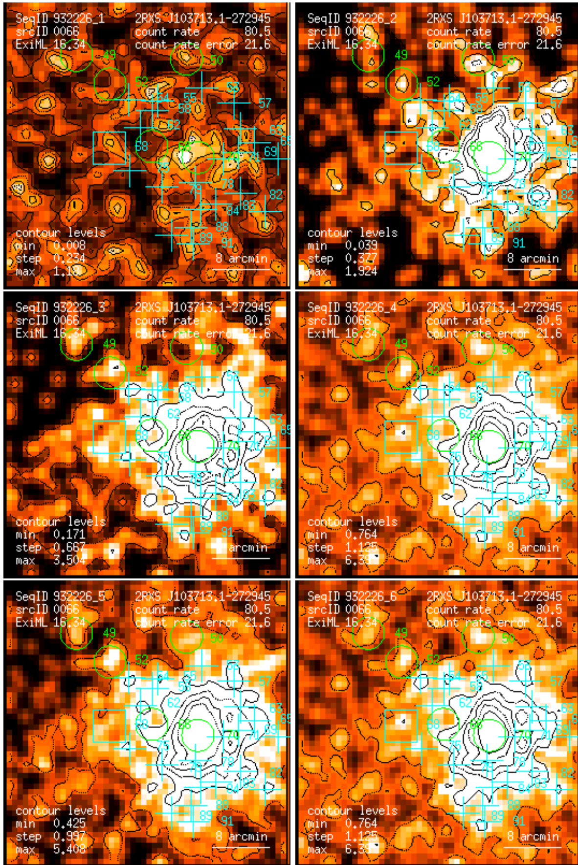
Figure 66: RASS 932226: detection 0066: band rate images, Gaussian filter: (1) PSPC channels 11 – 41, (2) 52 – 90, (3) 91 – 201, (4) 11 – 235, (5) 52 – 201, (6) 11 – 201. Broad band rates in counts/ks. Band rate contour levels in counts/ks/arcmin 2 .
